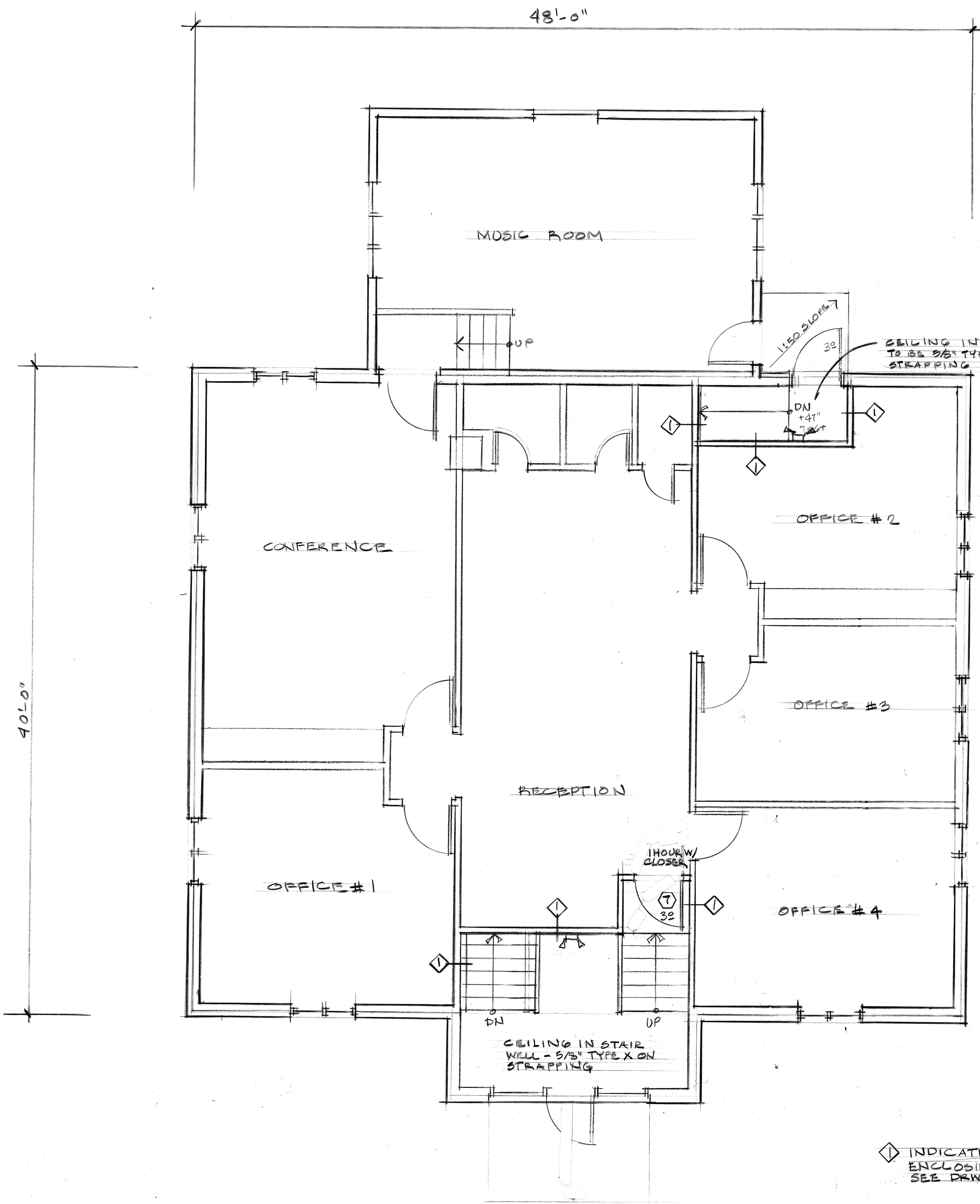
UPPER LEVEL FLOOR PLAN 1/4" = 1'-0" 2/384 SP
