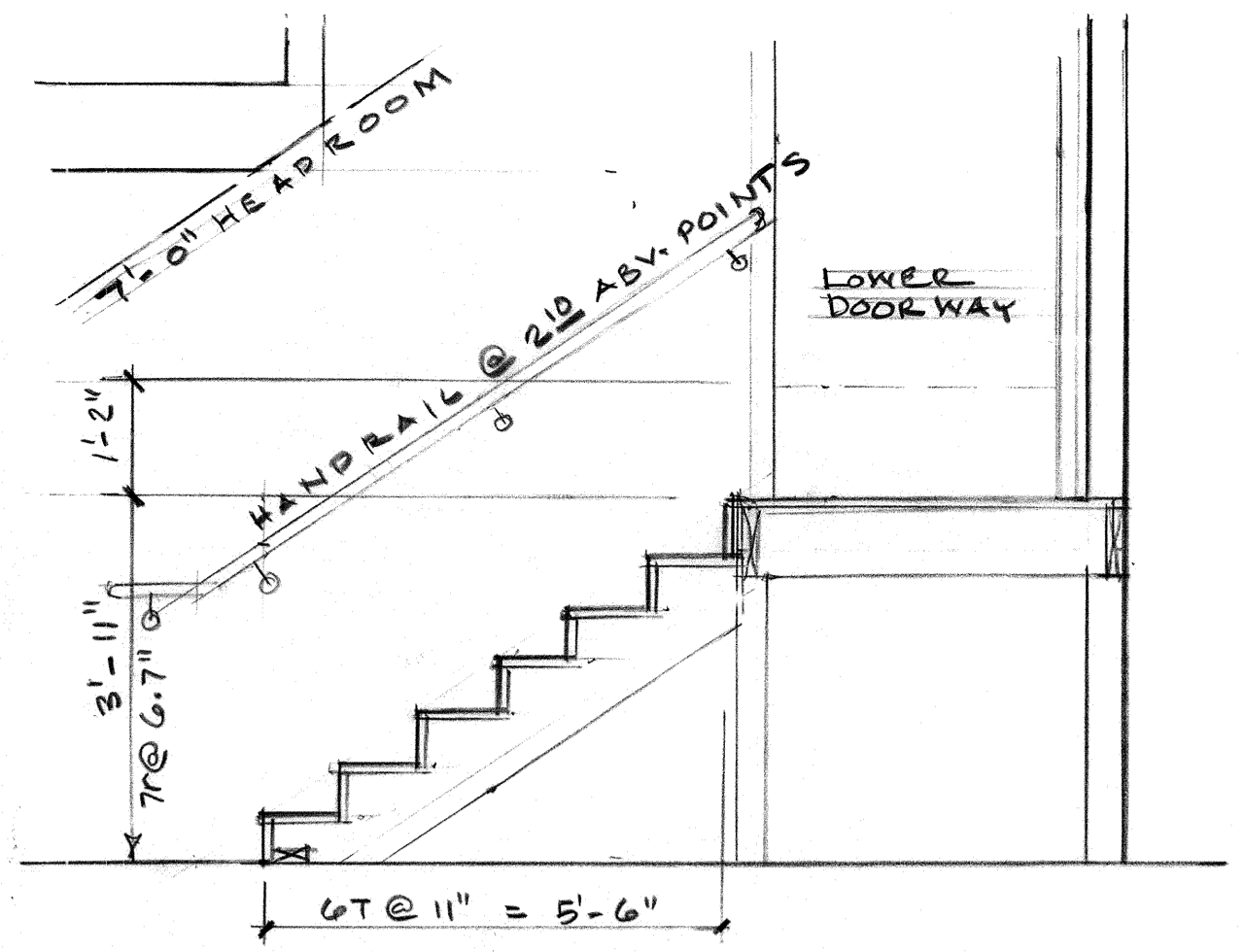
2 NEW EXIT STAIR 1/2" = 1'-0"
