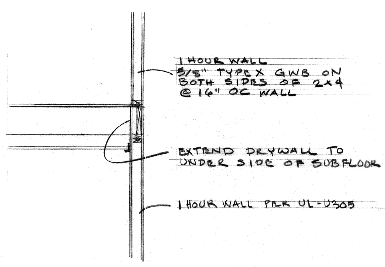
1 ONE HOUR WALL @ FLOOR DECK 1/2" = 1'-0"
