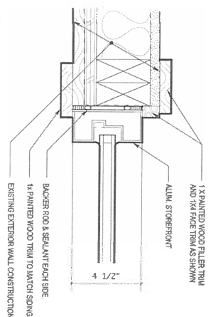
H2 J2 JAMB DETAIL (Head Similar)
