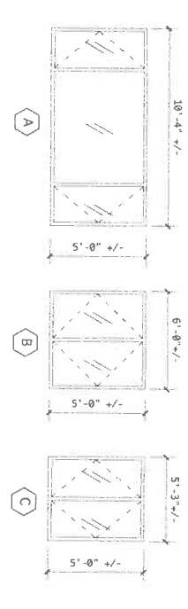
WINDOW TYPES
