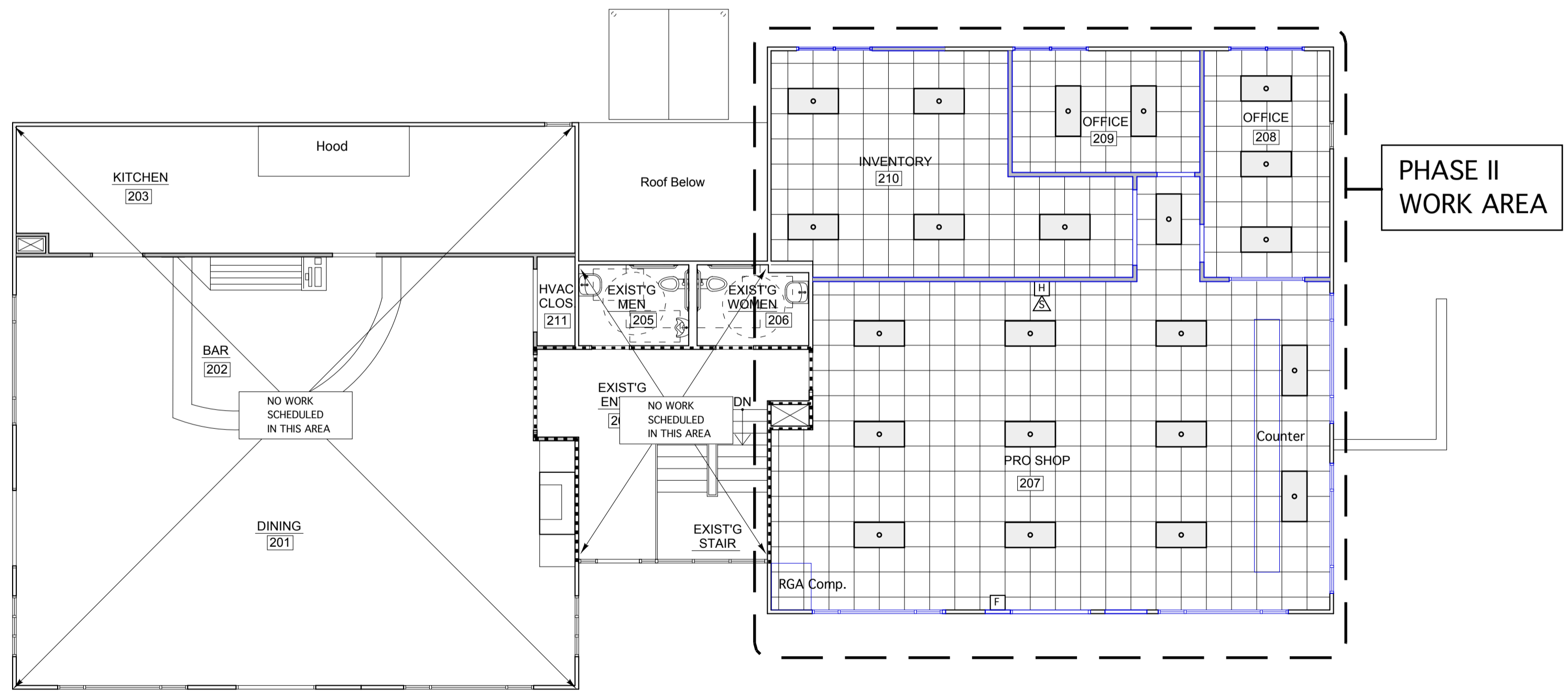
UPPER LEVEL CEILING PLAN
