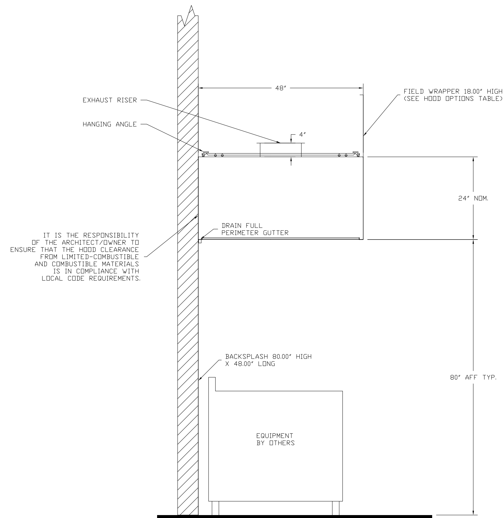
SECTION VIEW - MODEL 4824VHB-C HOOD - #2 (Dishwasher)
