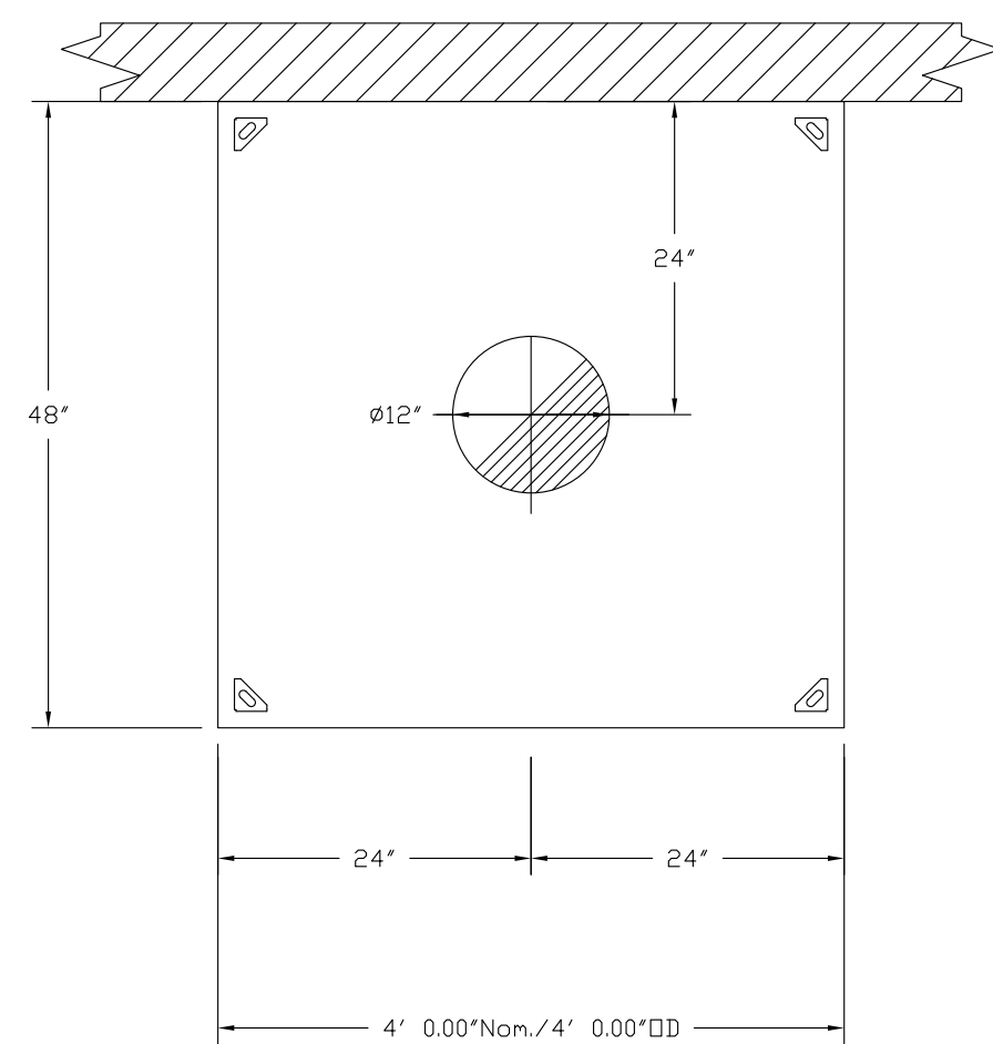
PLAN VIEW - Hood #2 (Dishwasher) 4' 0.00" LONG 4824VHB-C
