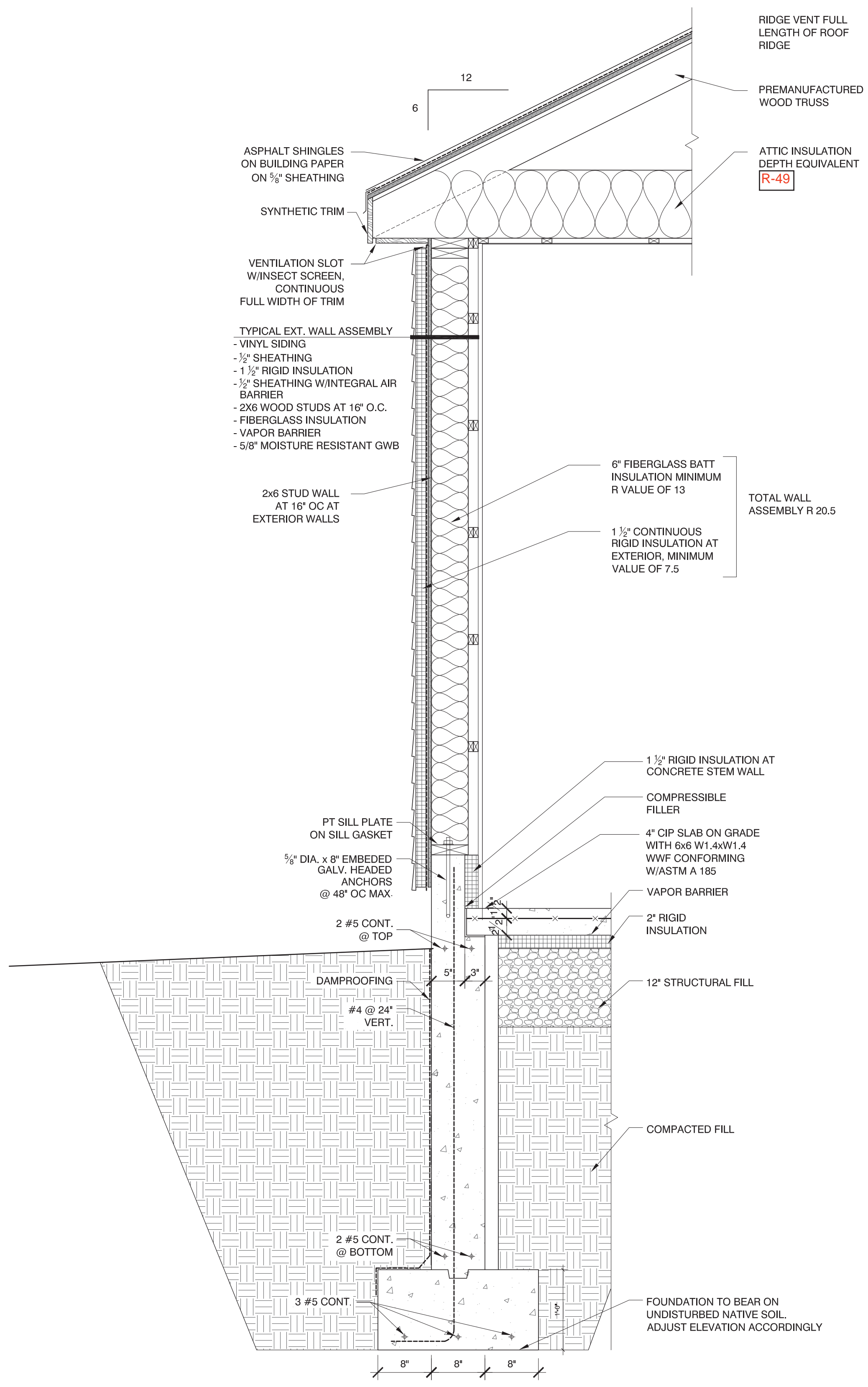
1 Wall Section 1"=1'-0"
