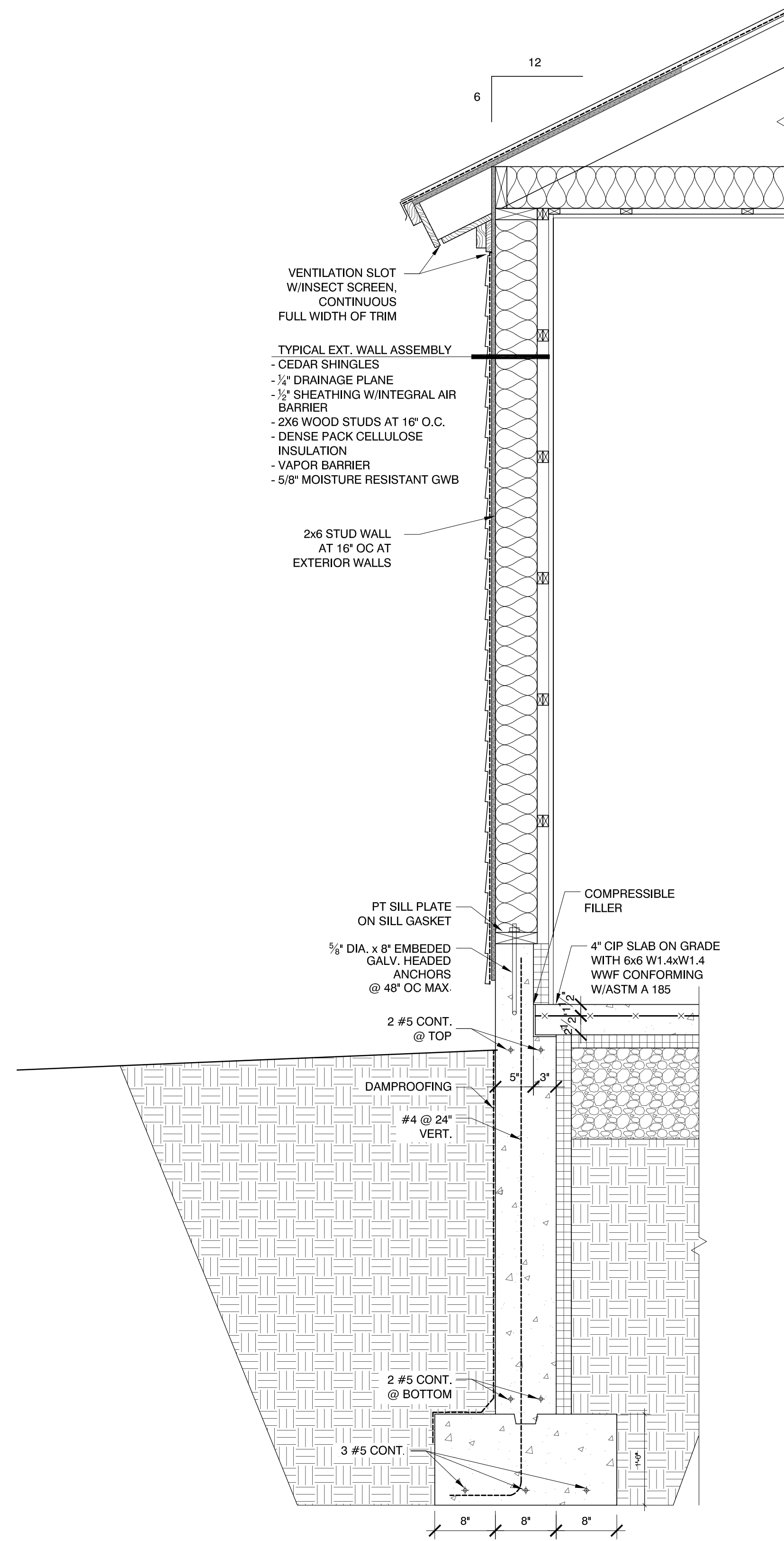
1 Wall Section 1"=1'-0"
