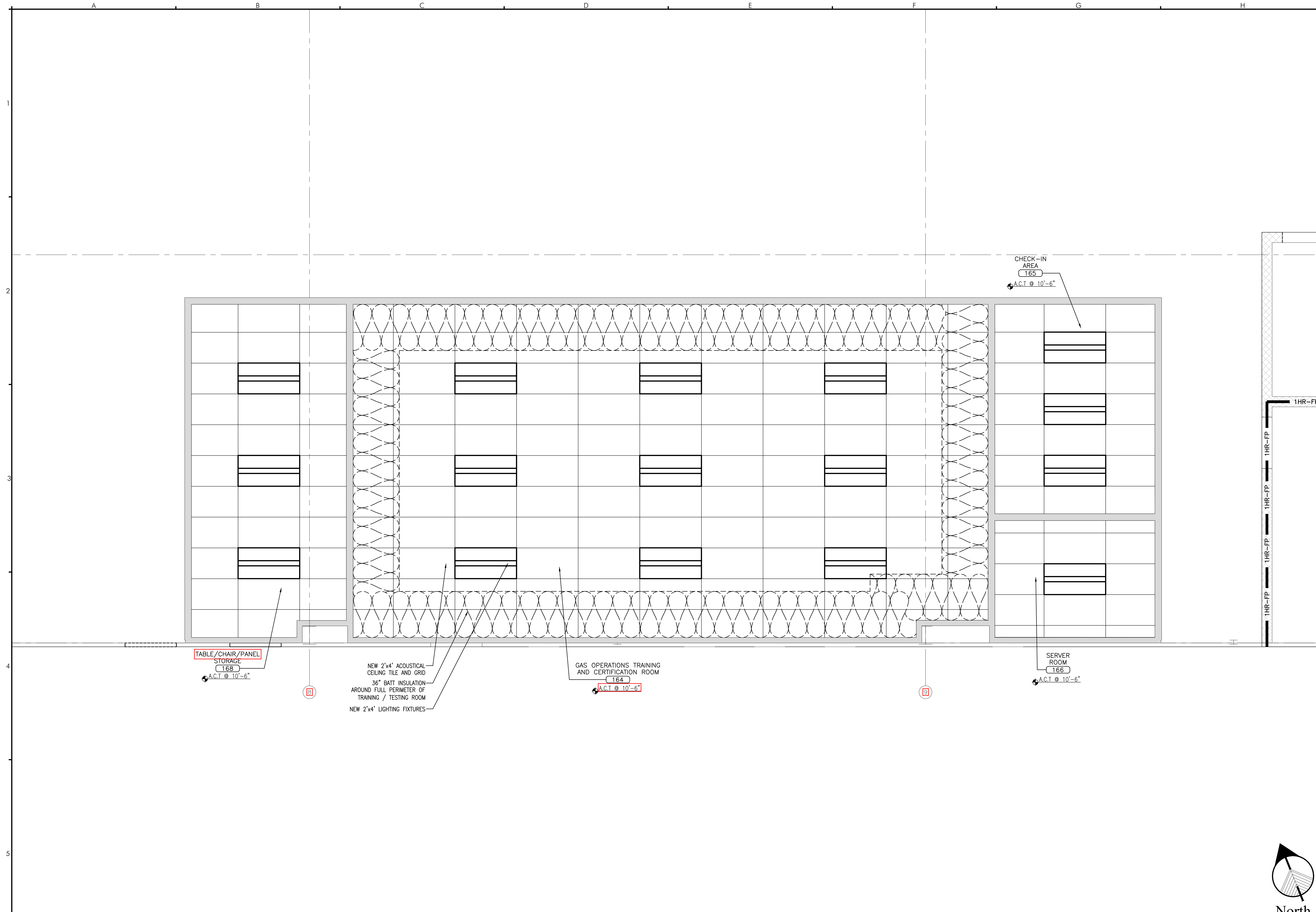
A5 ENLARGED TRAINING/TESTING ROOM REFLECTED CEILING PLAN REFERENCED FROM: A2.10 SCALE: 3/8" = 1'-0"
