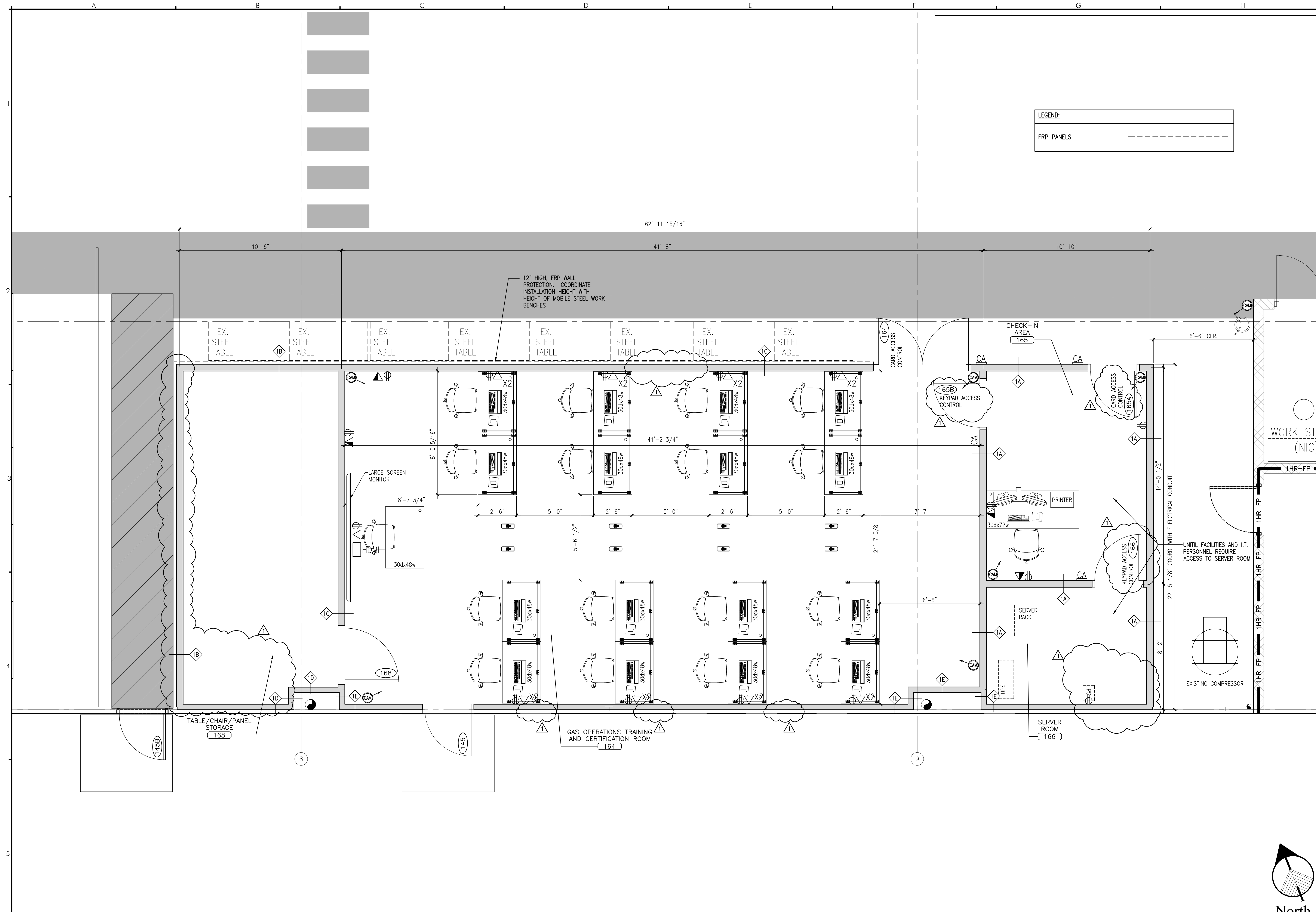
A5 ENLARGED CERTIFICATION / TESTING FURNITURE PLAN REFERENCED FROM: A1.12 SCALE: 3/8" = 1'-0"
