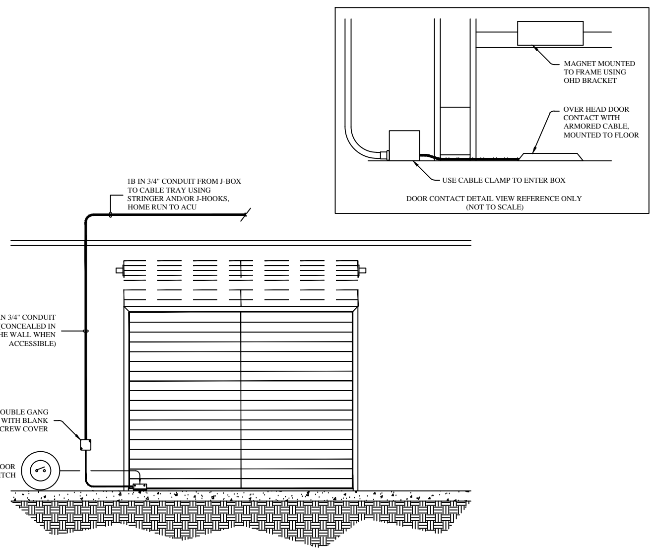
114 INSTALLATION GUIDELINE #114 OVERHEAD DOOR WITH SURFACE MOUNT DOOR CONTACT
