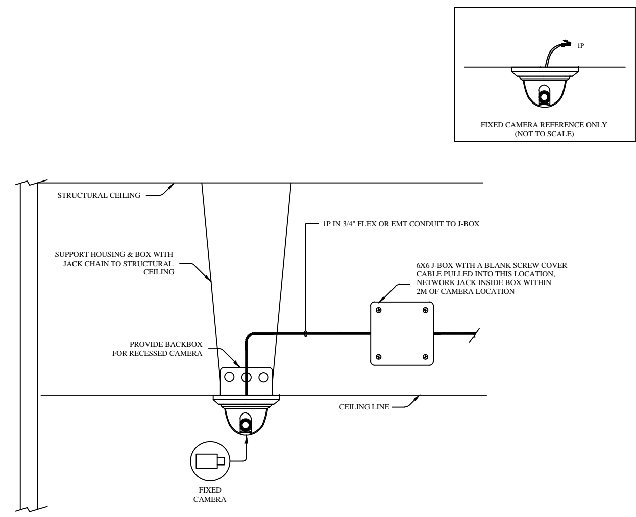
01 INSTALLATION GUIDELINE #01 INTERIOR/ EXTERIOR IP FIXED CAMERA MOUNTED FLUSH IN CEILING
