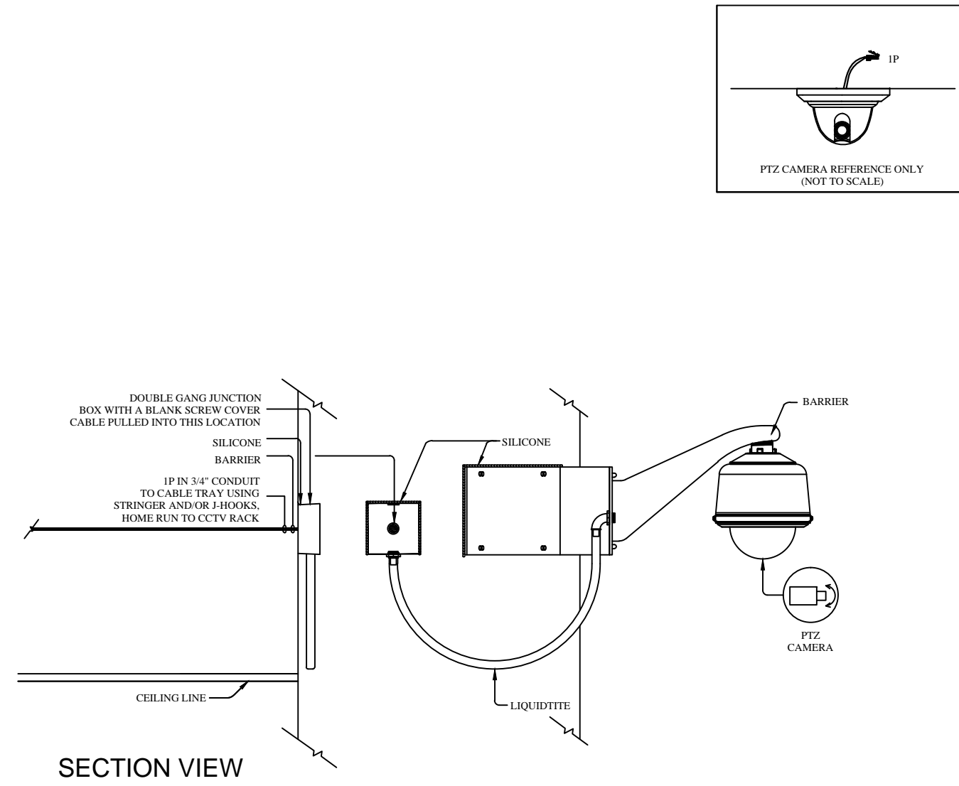
32 INSTALLATION GUIDELINE #32 EXTERIOR IP WALL CORNER MOUNTED PTZ CAMERA
