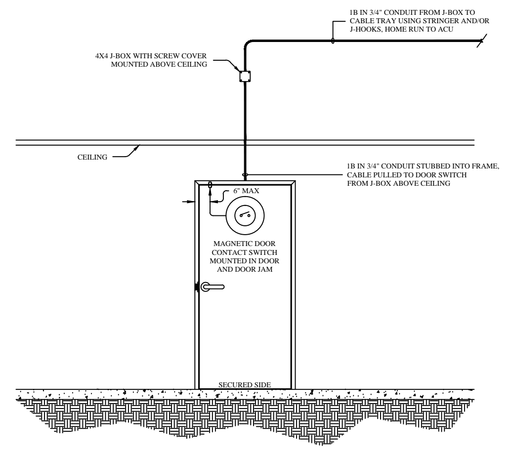
101 INSTALLATION GUIDELINE #101 SINGLE DOOR WITH RECESSED DOOR CONTACT
