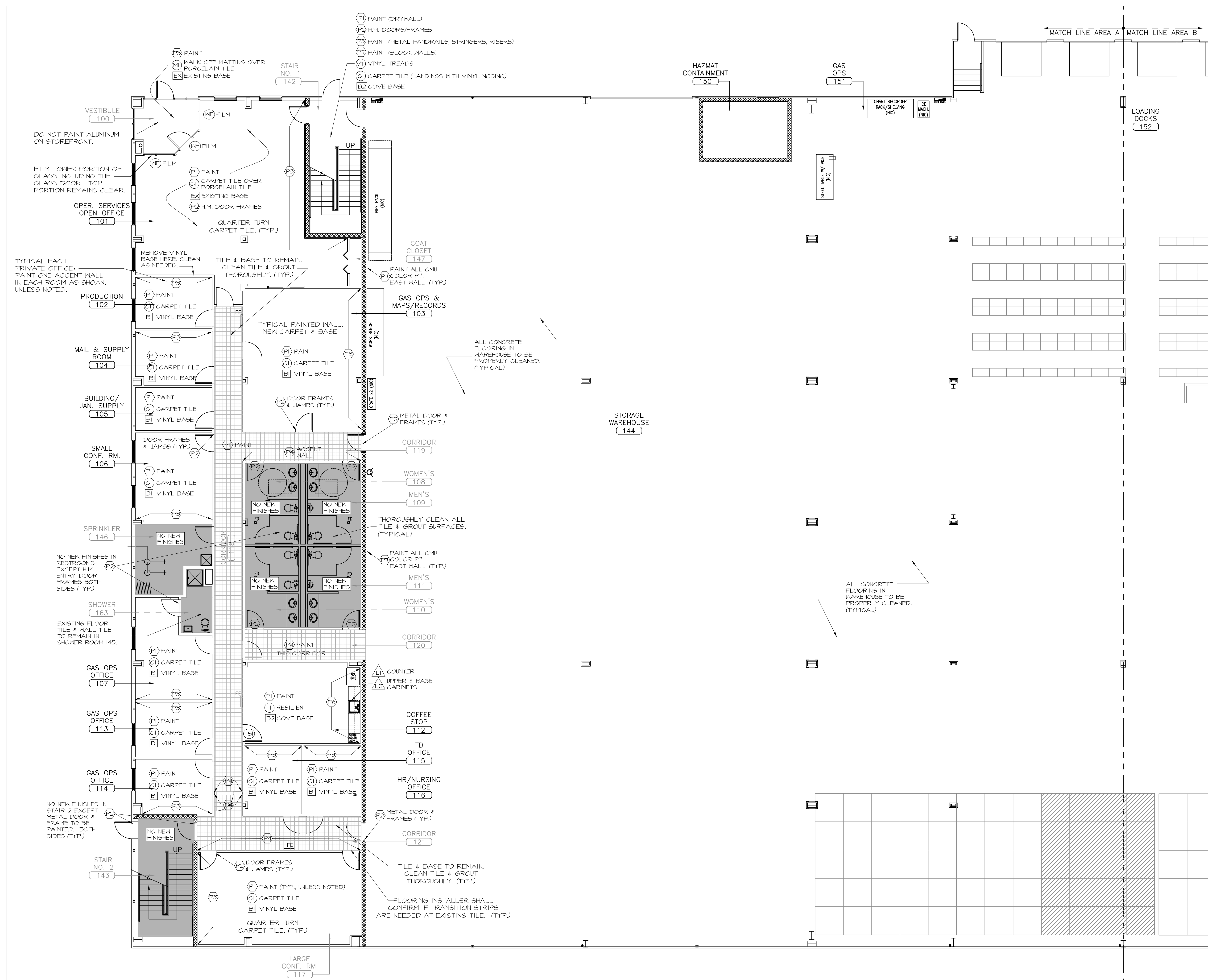
A FINISH PLAN - PARTIAL FRONT (AREA A) 1/8" = 1'-0"
