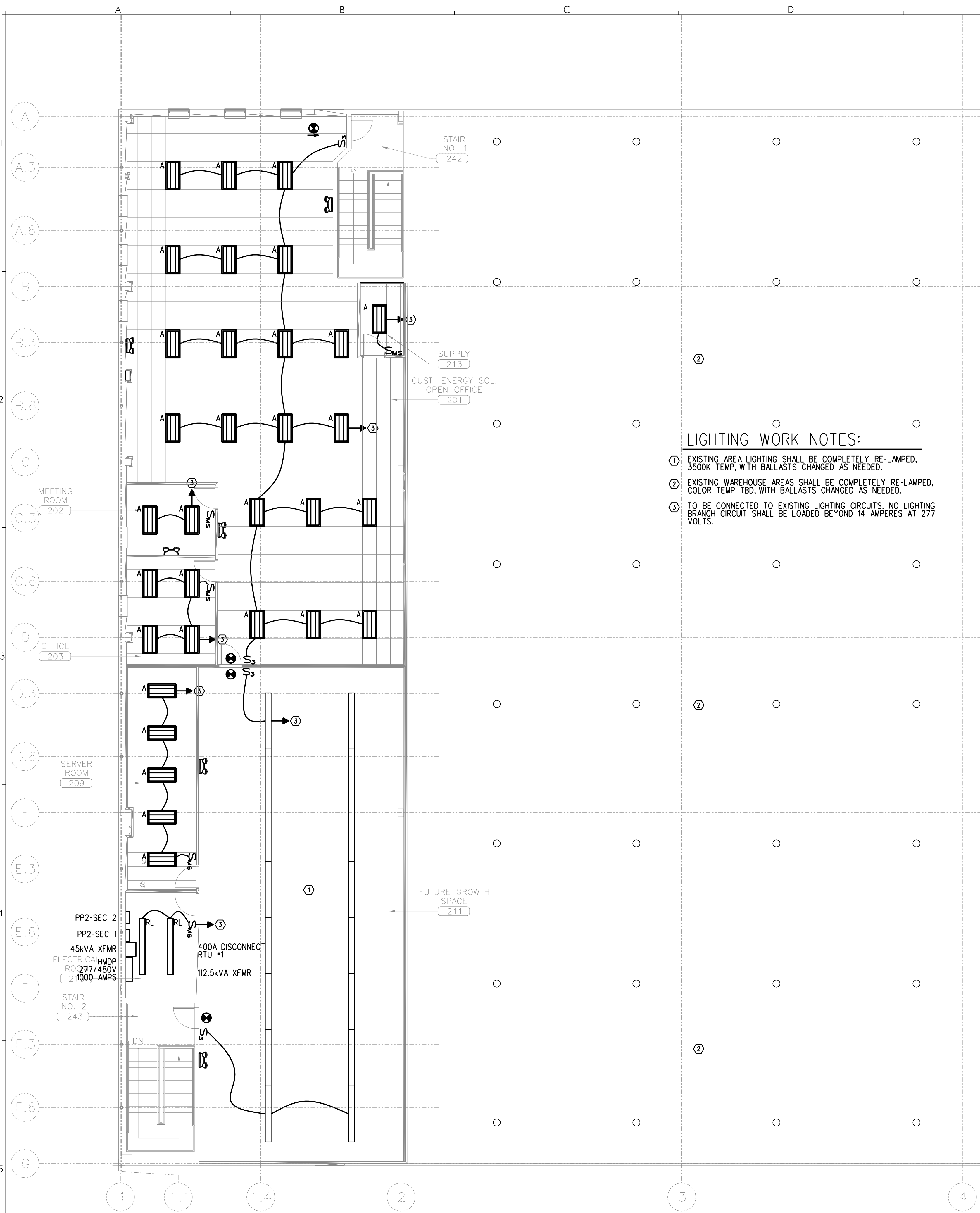
E1 NEW SECOND FLOOR LIGHTING PLAN- AREA "A" SCALE: 1/8" = 1'-0"
