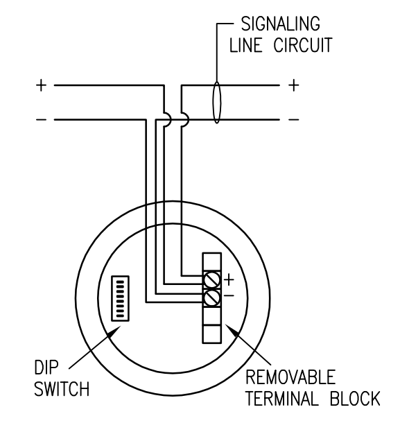
5192SD SMOKE DETECTOR WIRING DETAIL SCHEMATIC: NO SCALE
