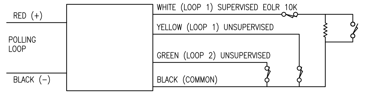
4193SN TWO ZONE SIM WIRING DETAIL SCHEMATIC: NO SCALE
