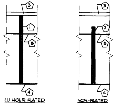
3 PARTITION WALL TYPES SCALE: 1/4"=1'-0"
