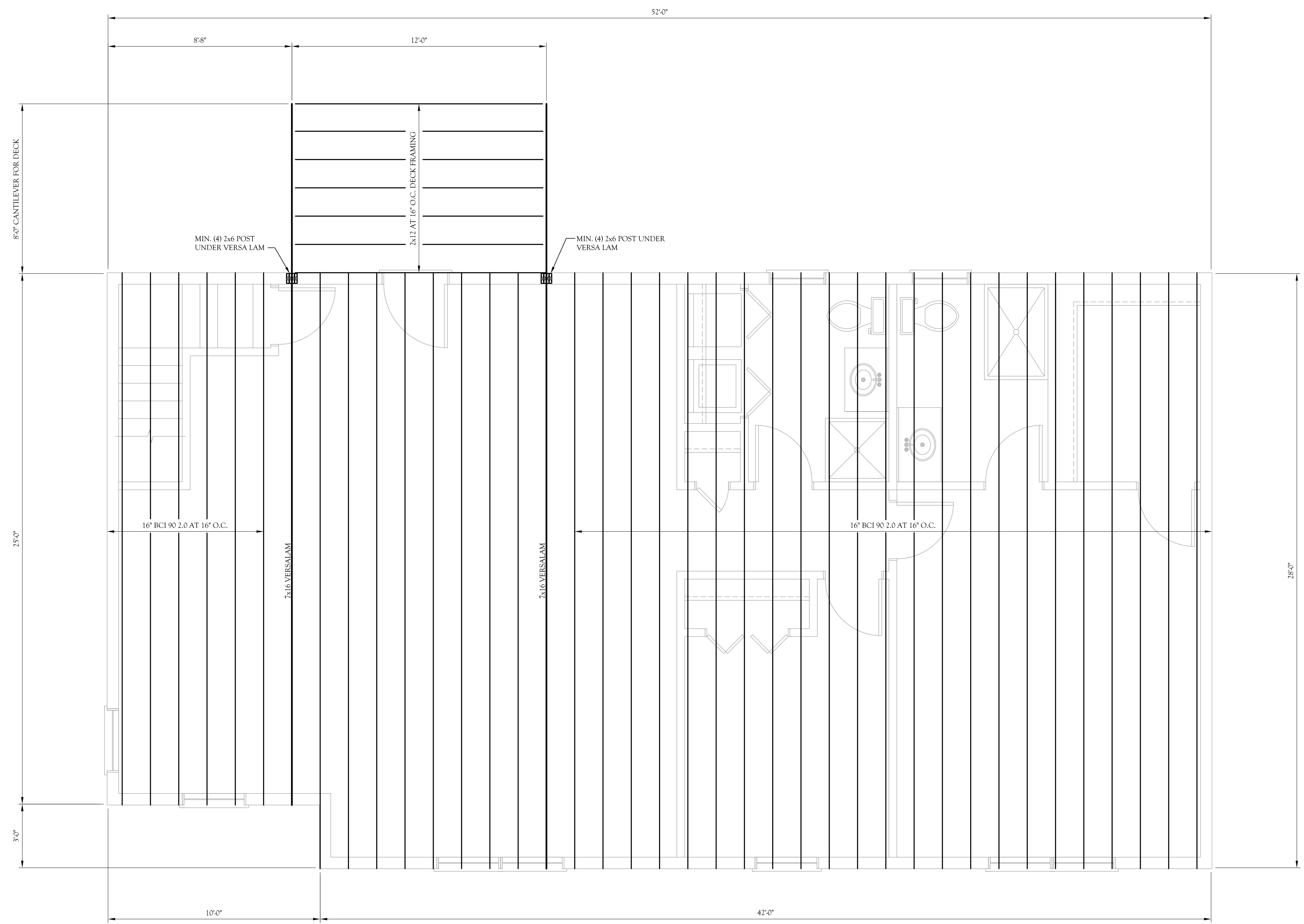
2nd FLOOR FRAMING PLAN SCALE: 1/8" = 1'-0"
