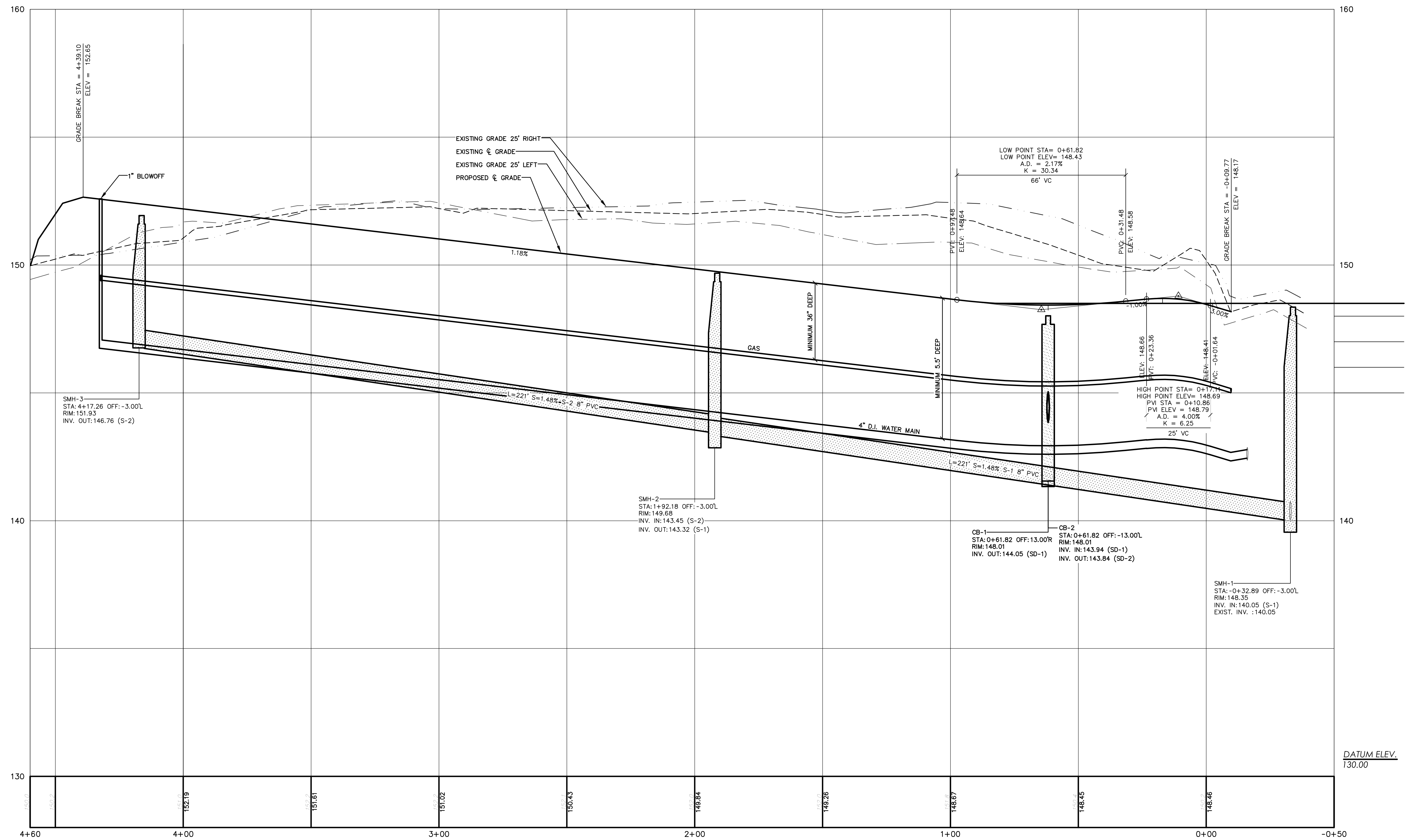
PROFILE: PROPOSED ROAD STA. -0+50 TO STA. 4+60 SCALE: 1"=20' HORIZ. 1"=2' VERT.
