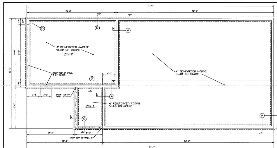
FOUNDATION PLAN 1/4" = 1'-0"
