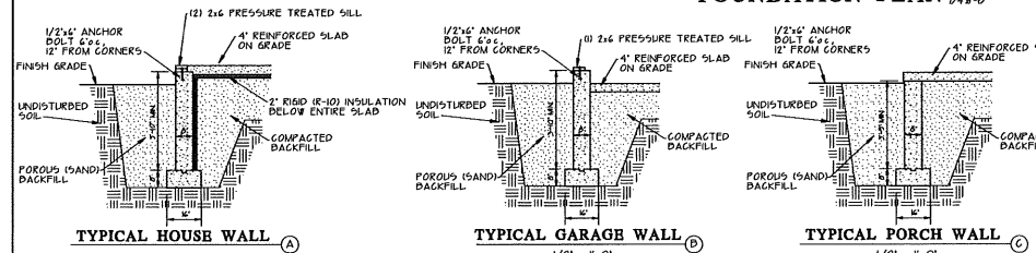
TYPICAL HOUSE WALL 1/2" = 1'-0"
