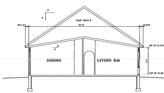
BUILDING SECTION 1/4" = 1'-0"
