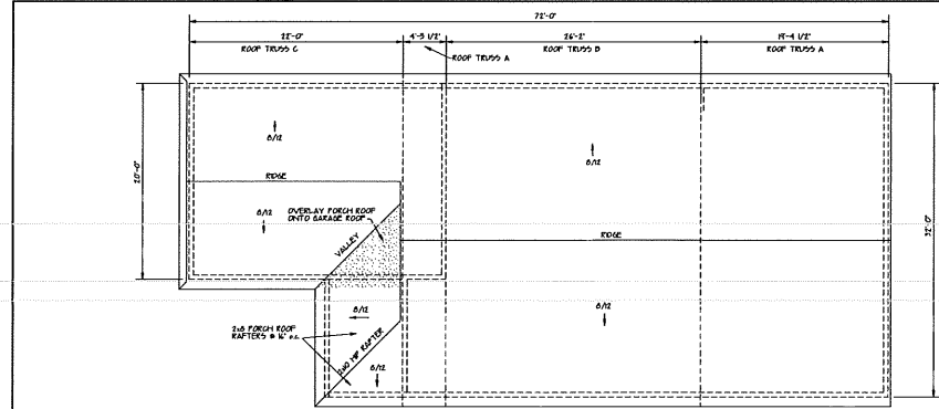
ROOF PLAN 3/16" = 1'-0"
