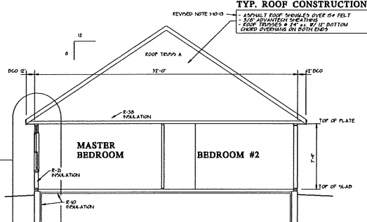
BUILDING SECTION 1/4" = 1'-0"
