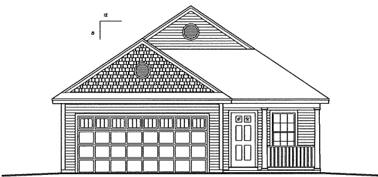
FRONT ELEVATION 1/4" = 1'-0"
