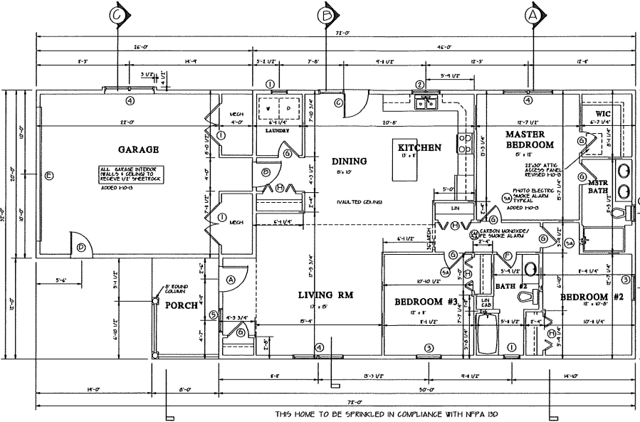
FLOOR PLAN 1/4" = 1'-0"
