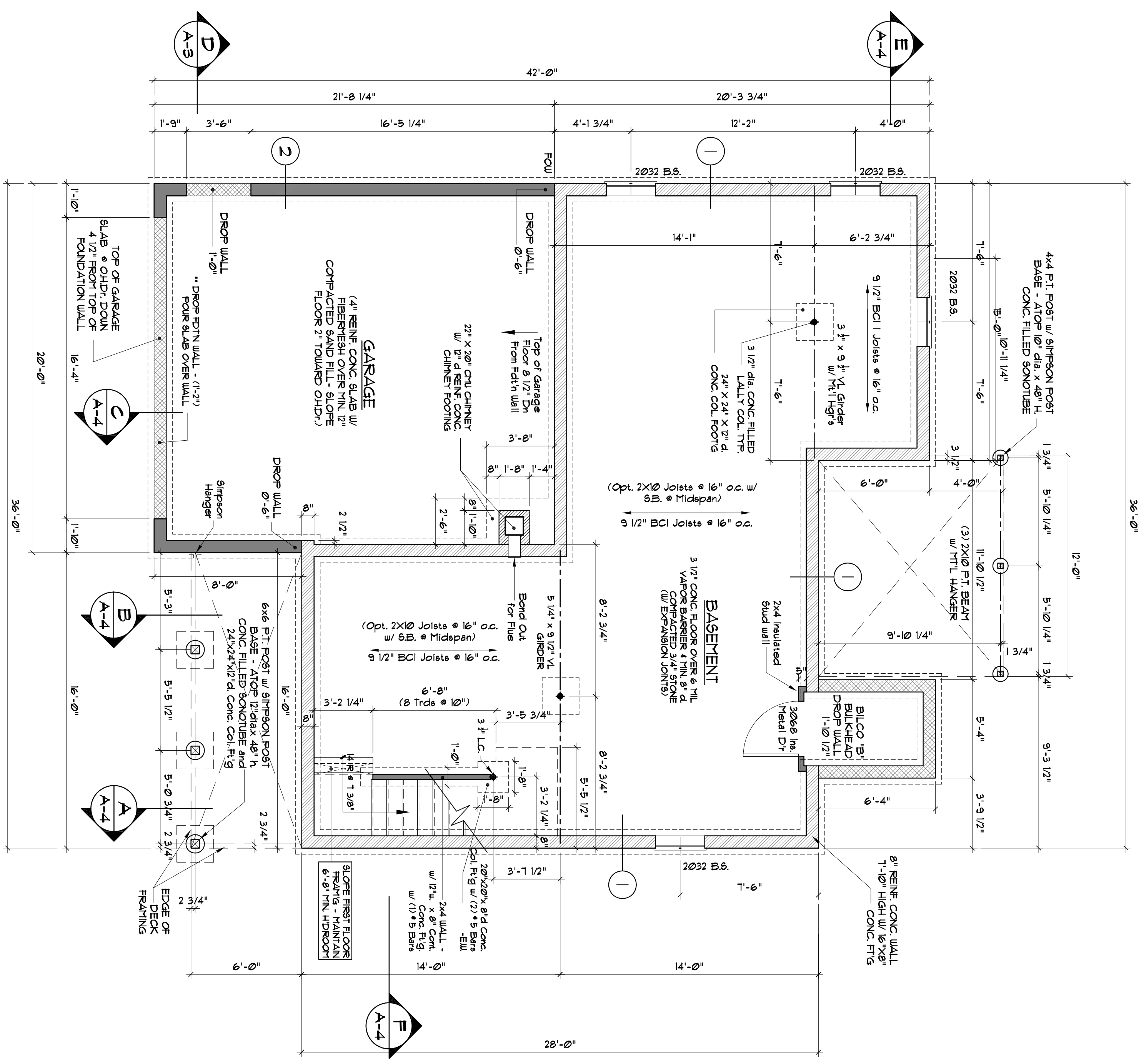
FOUNDATION / BASEMENT PLAN Scale: 1/4" = 1'-0"
