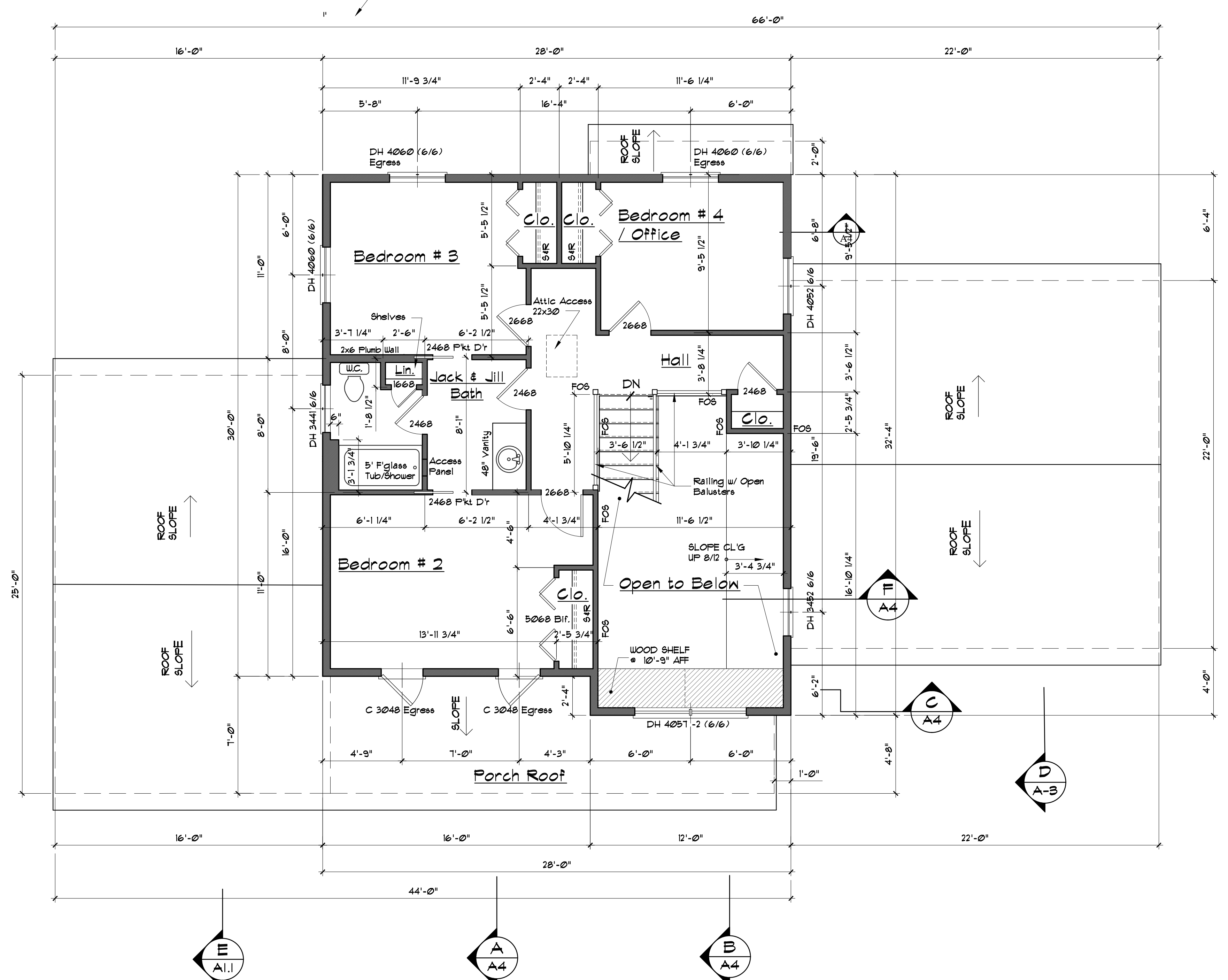
SECOND FLOOR PLAN - Colonial w/ First Floor M. Bath Scale: 1/4" = 1'-0" (654 s.f.)
