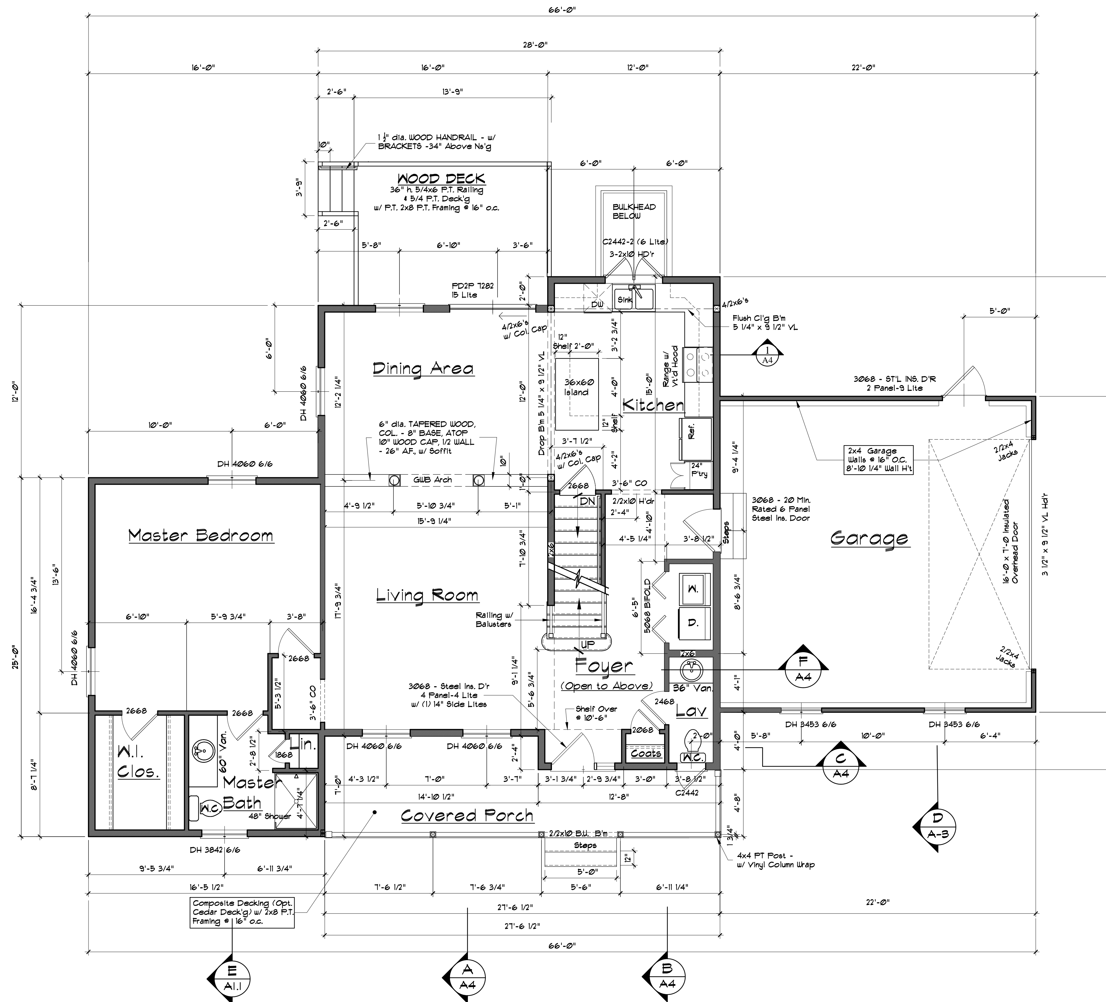
FIRST FLOOR PLAN - Colonial w/ First Floor M. Bath Scale: 1/4" = 1'-0" Total Area (1,951 s.f.) (1,297 s.f.)
