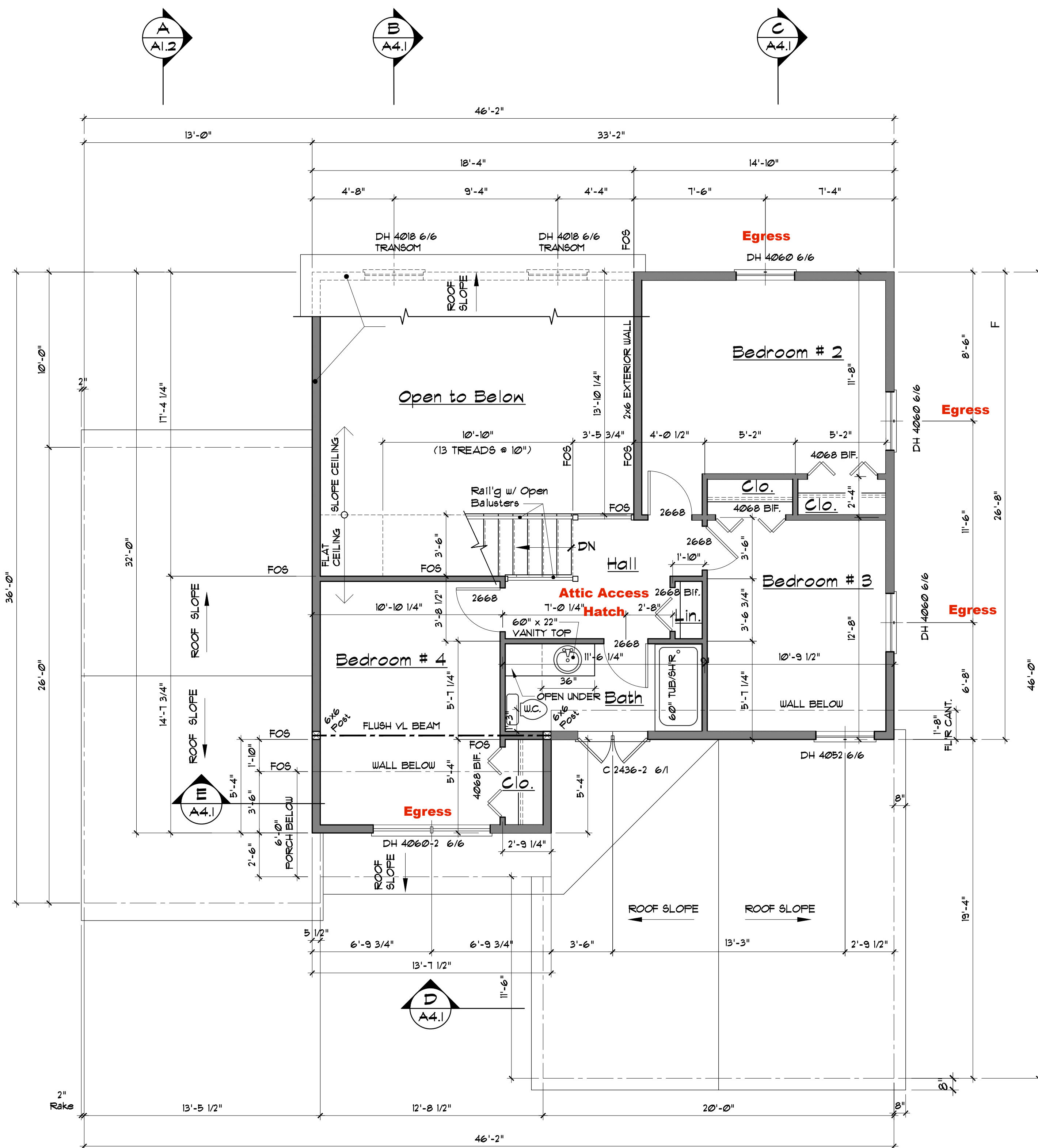
SECOND FLOOR PLAN (703 s.f.) Scale: 1/4" = 1'-0"
