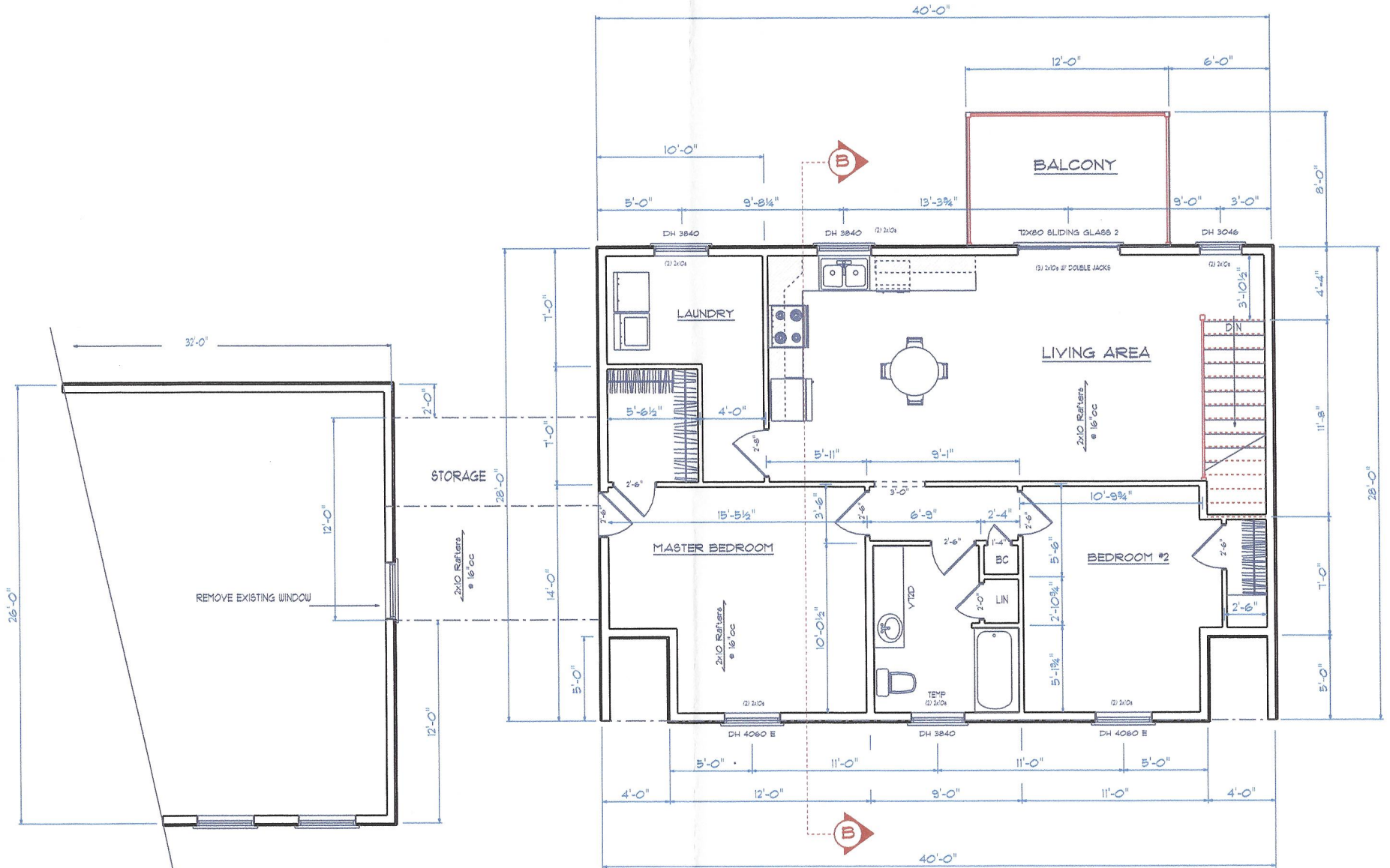
Upper Floor Plan 1/4" = 1'-0"
