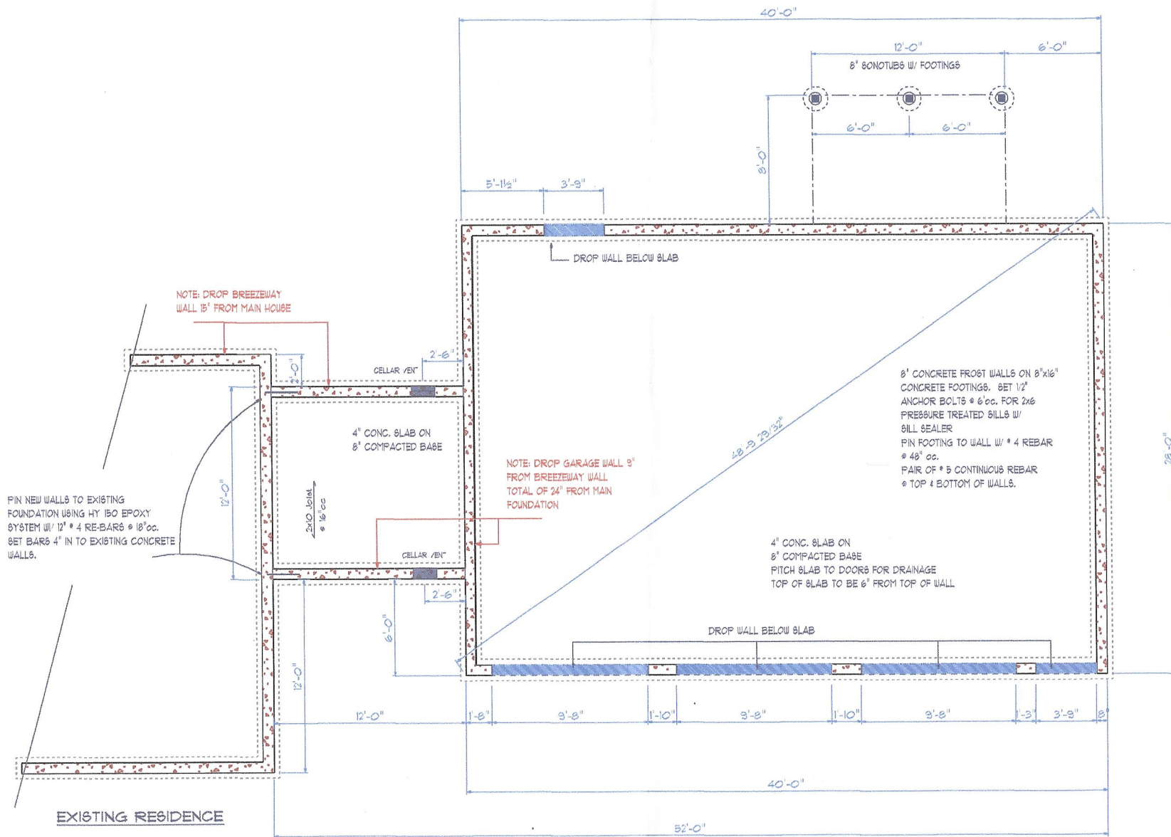
Foundation Plan 1/4" = 1'-0"
