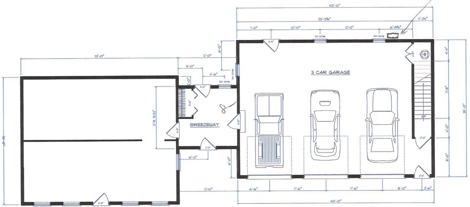
Lower Floor Plan
