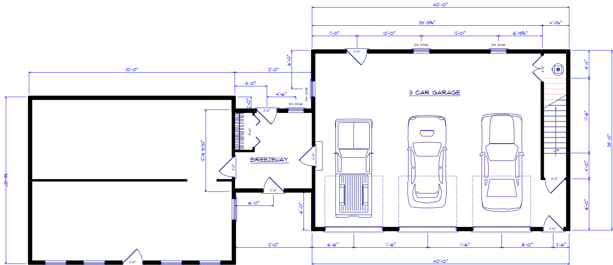
Lower Floor Plan
