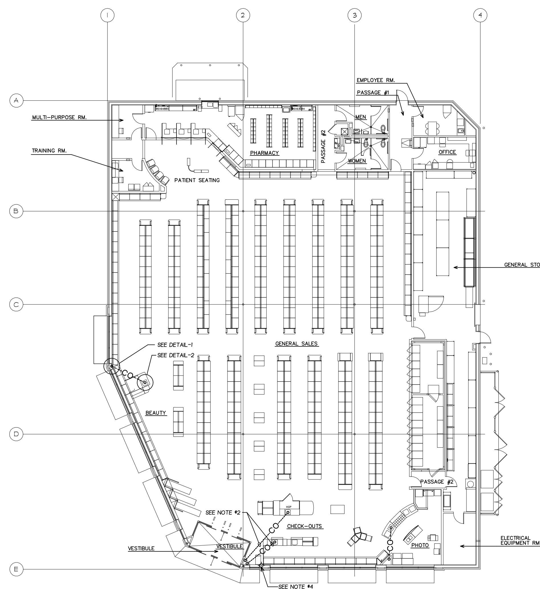
FLOOR PLAN - SPARE CONDUIT SCALE: 1/16" = 1'-0"
