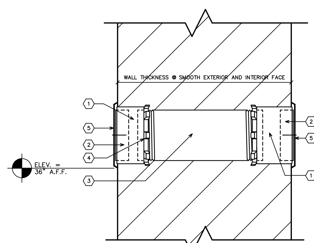
WALL SECTION AT SLEEVE IN ELECTRICAL EQUIPMENT ROOM N.T.S. (SEE SPARE CONDUIT NOTE 3)
