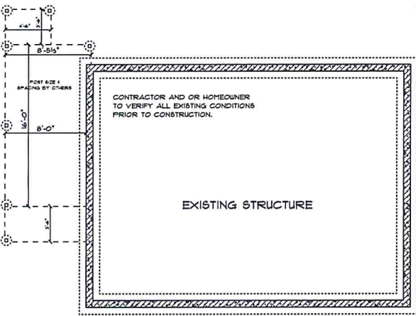
FOUNDATION SCALE: 1/4" = 1'-0"
