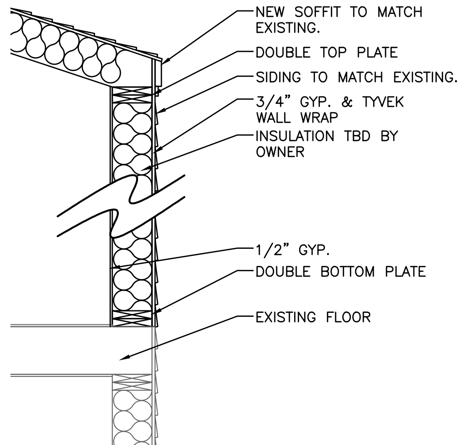
3 NEW WALL DETAIL SCALE: 1" = 1-0"
