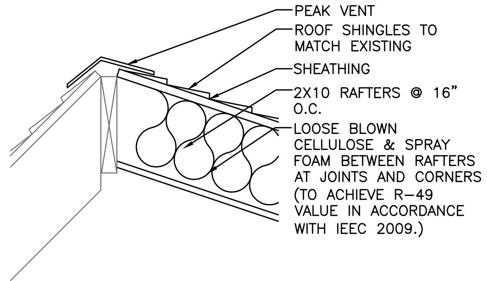
2 ROOF PEAK DETAIL SCALE: 1" = 1-0"
