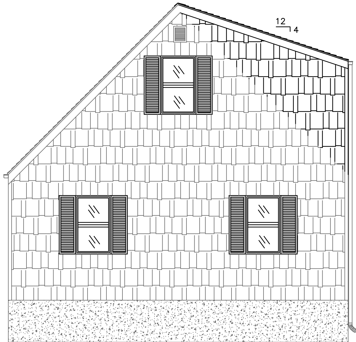
1 RIGHT ELEVATION — NORTH WEST SIDE SCALE: 1/4" = 1-0"
