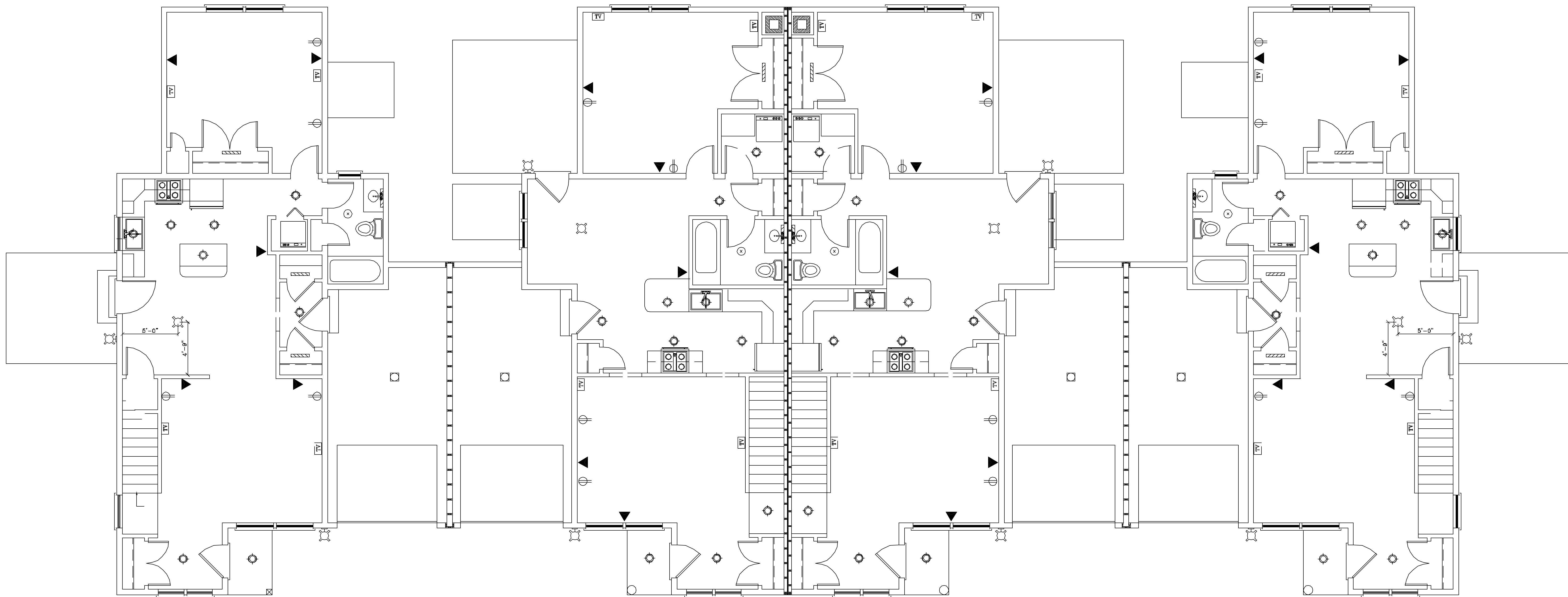
FIRST FLOOR ELECTRICAL PLAN SCALE: 1/4" = 1'-0"
