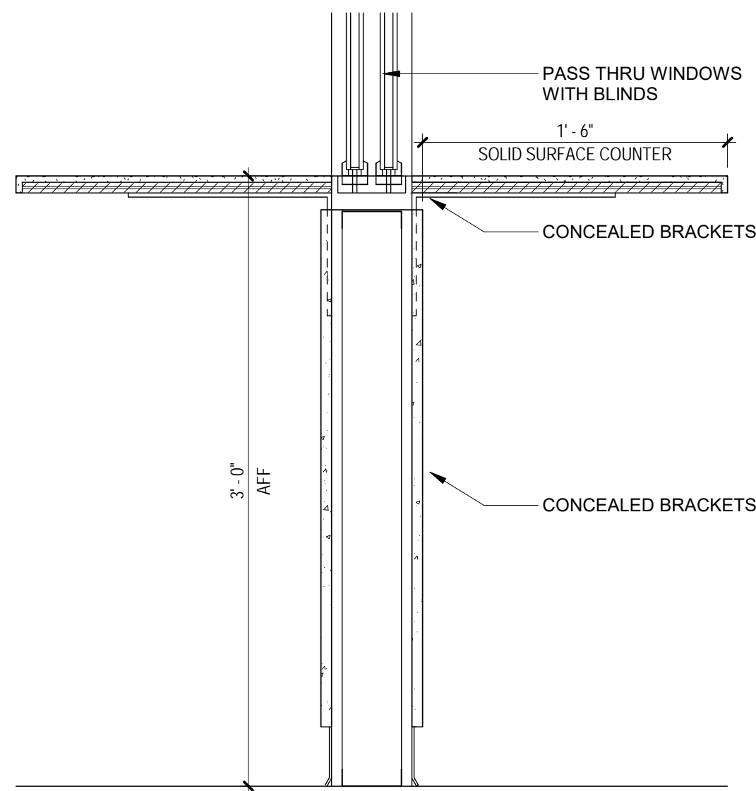
D3 COUNTER - PASS THRU WINDOW 1 1/2" = 1'-0"
