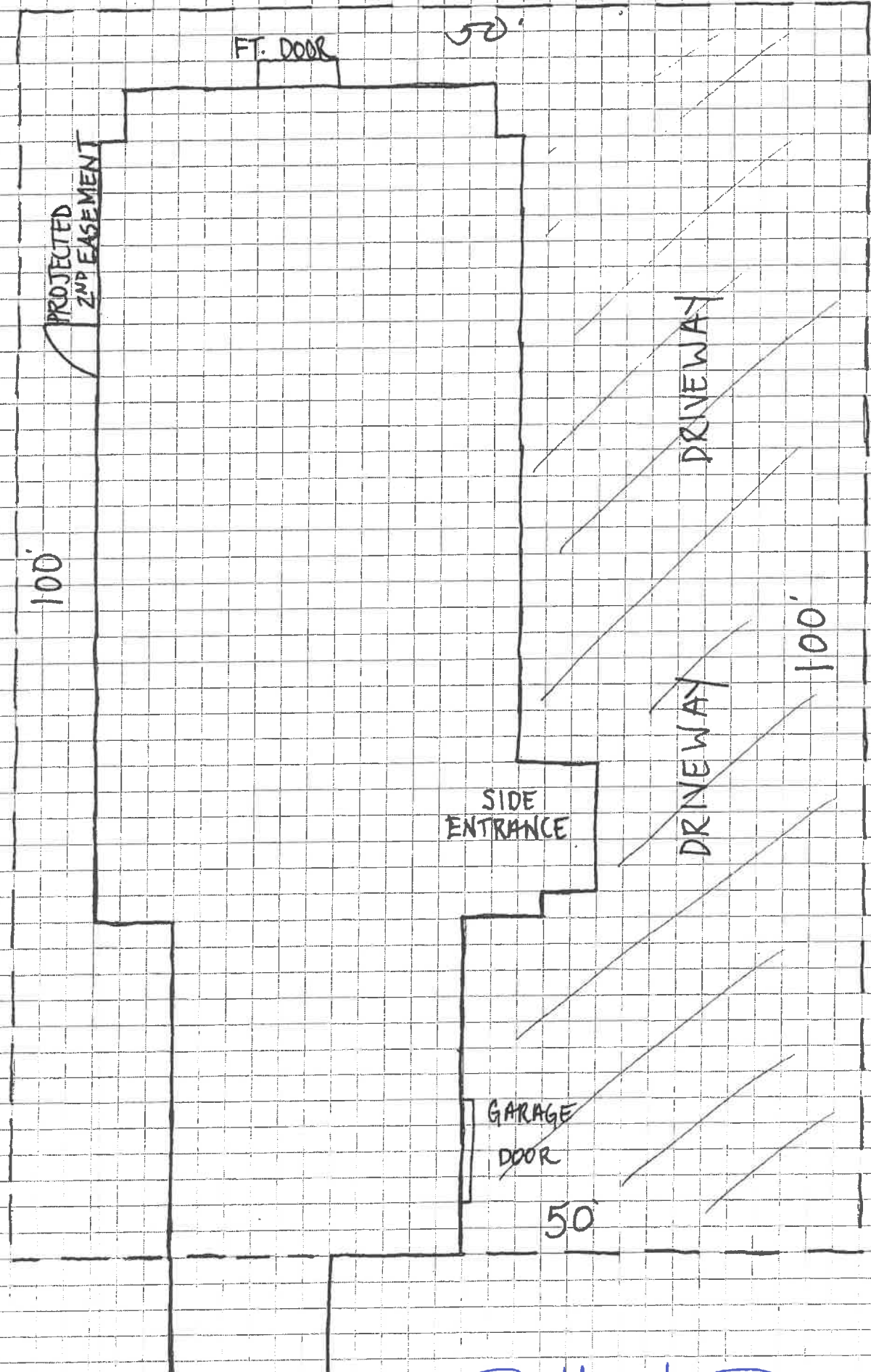
120 Allen Avenue, Portland PLOT PLAN
