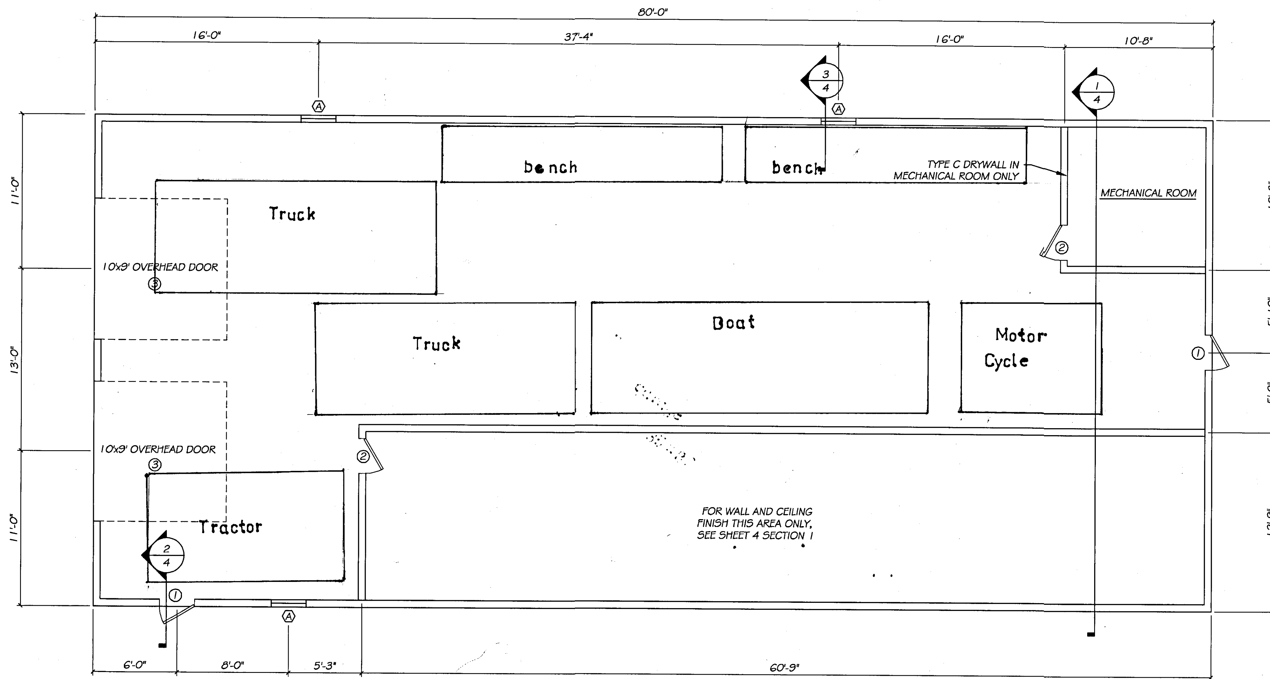
FLOOR PLAN
