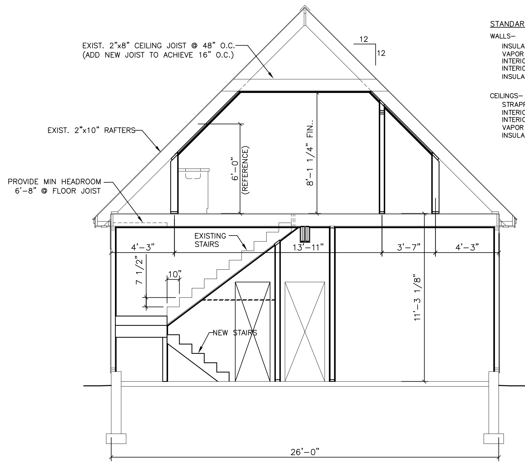
A SECTION @ GARAGE A1 SCALE: 1/4"=1'-0"
