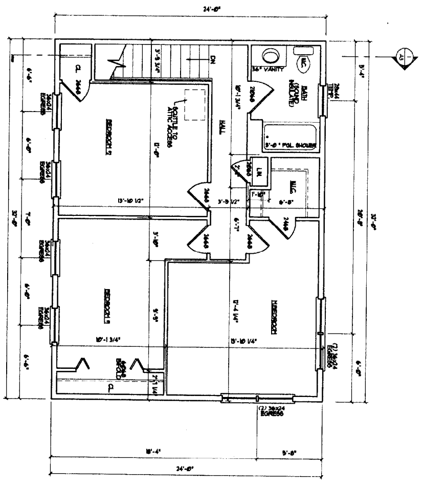
SECOND FLOOR PLAN SCALE: 1/4\"/>
