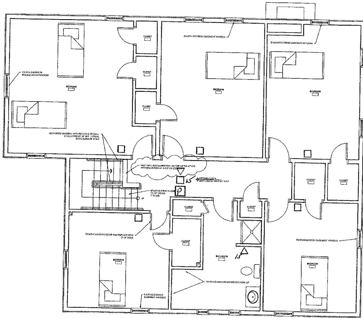
1 SECOND FLOOR PLAN
