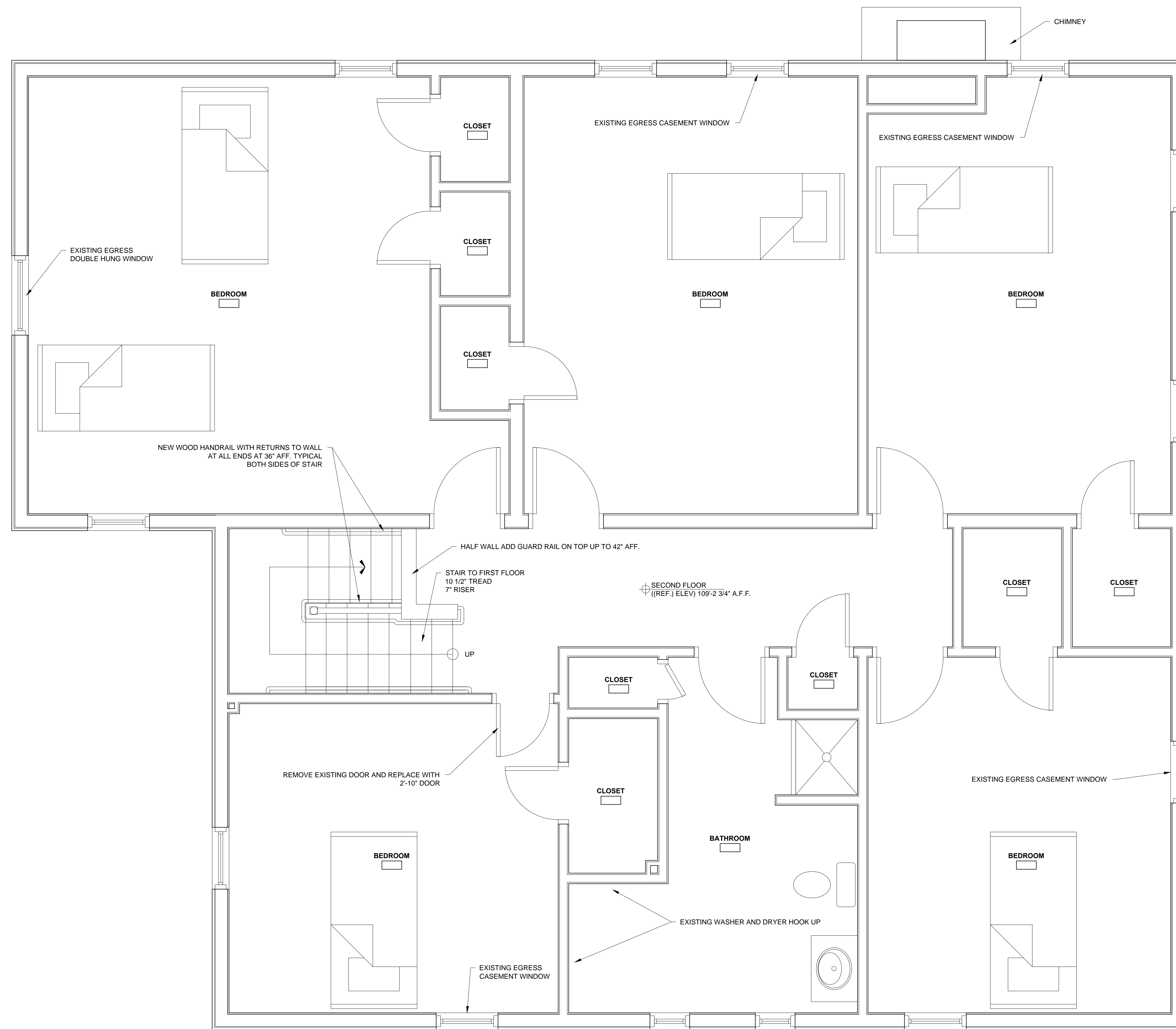
1 SECOND FLOOR PLAN 1/2" = 1'-0"
