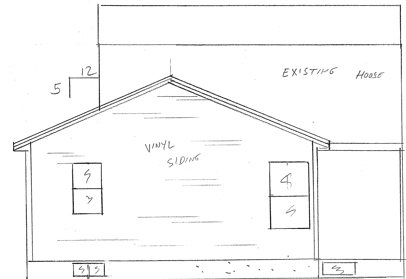
LEFT END ELEVATION
