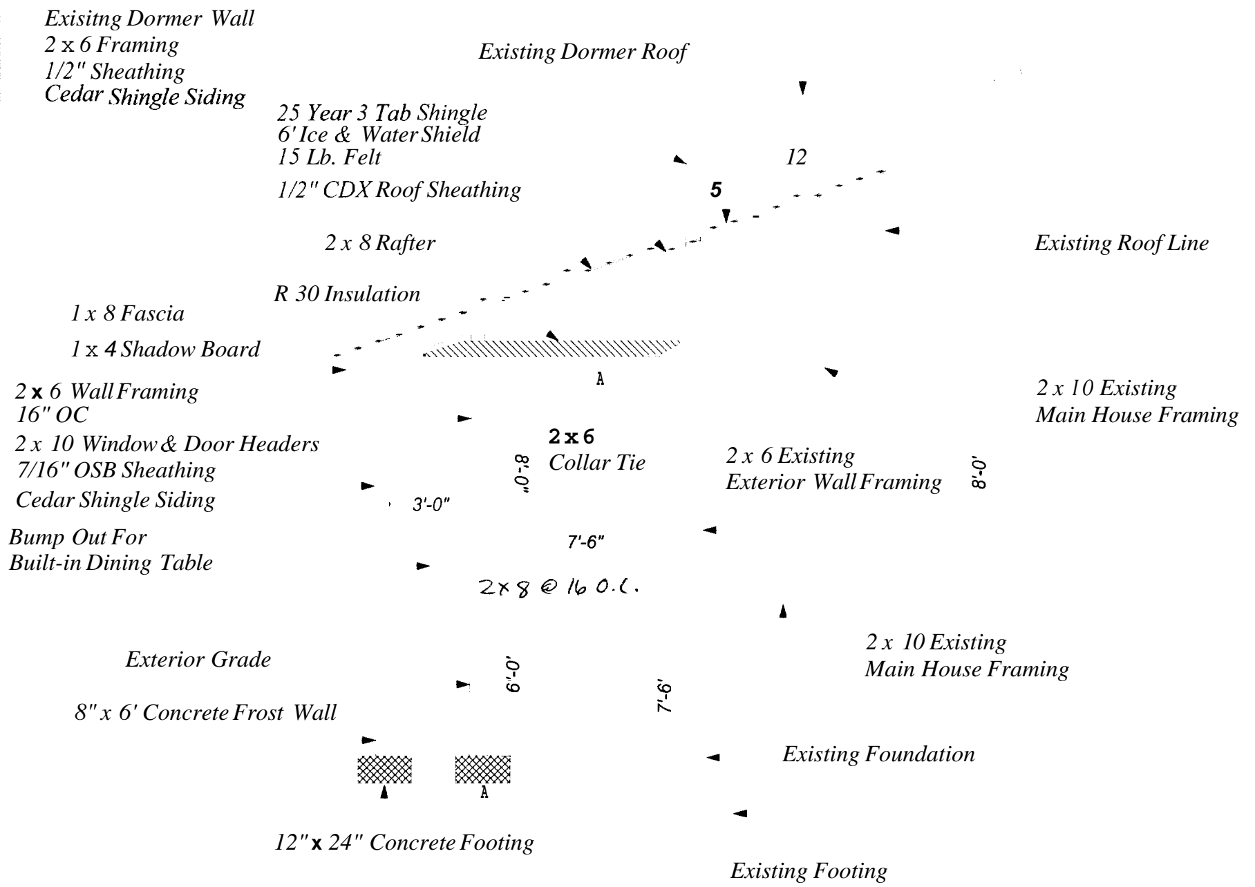
A-2 Cross Section Existing Main House & New Addition
