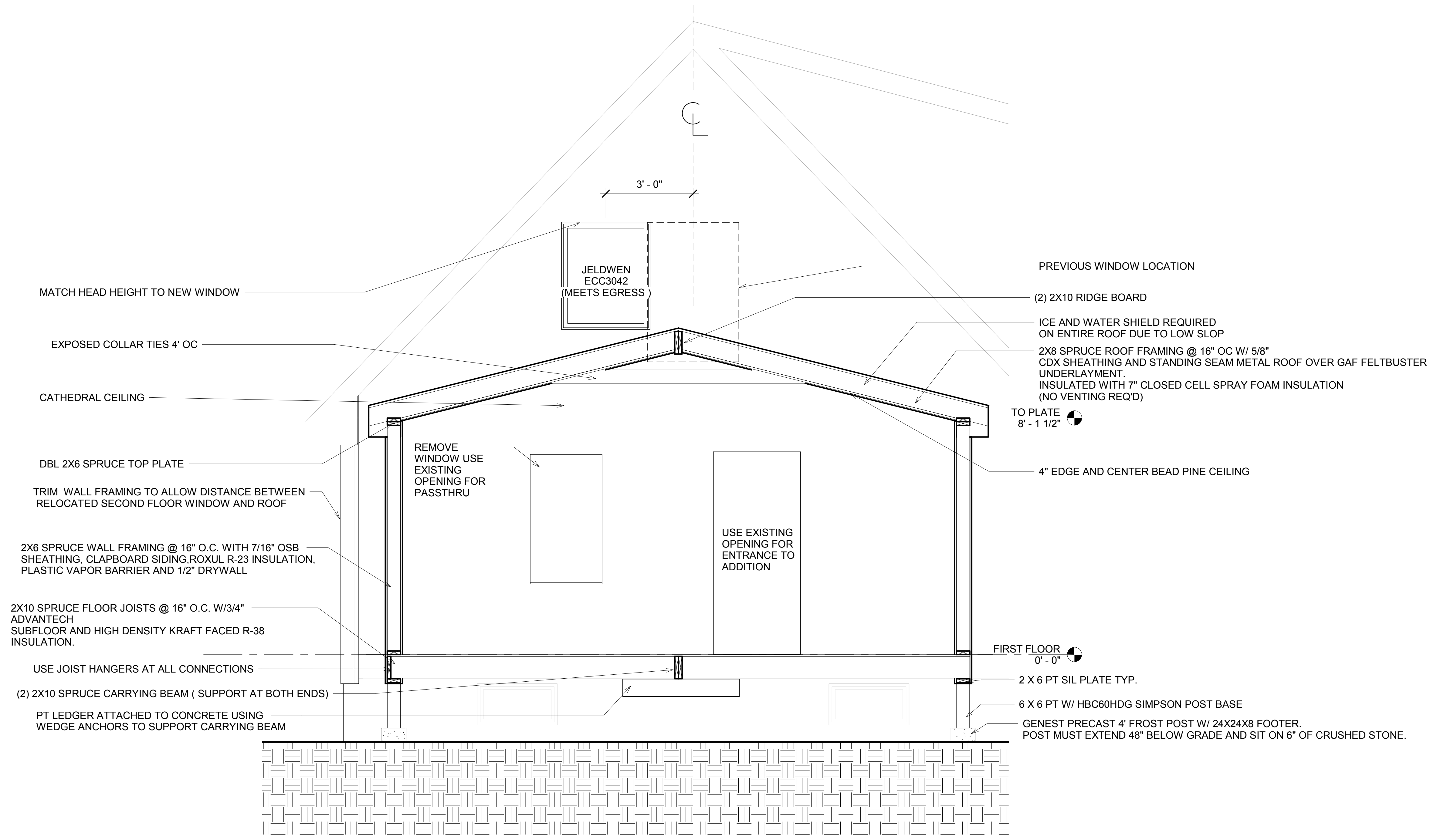
1 Section 1 1/2" = 1'-0"
