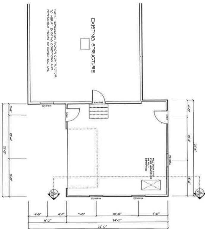
MAIN FLOOR SCALE: 1/4" = 1'-0"
