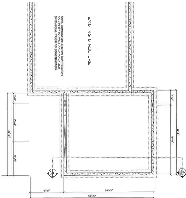
FOUNDATION SCALE: 1/4" = 1'-0"
