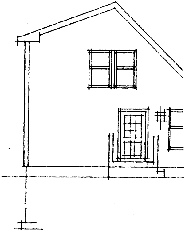
LEFT ELEVATION
