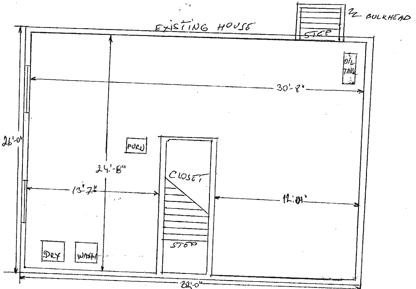
BASEMENT FLR PLAN EXISTING SCALE = 1/4" = 1'-0"
