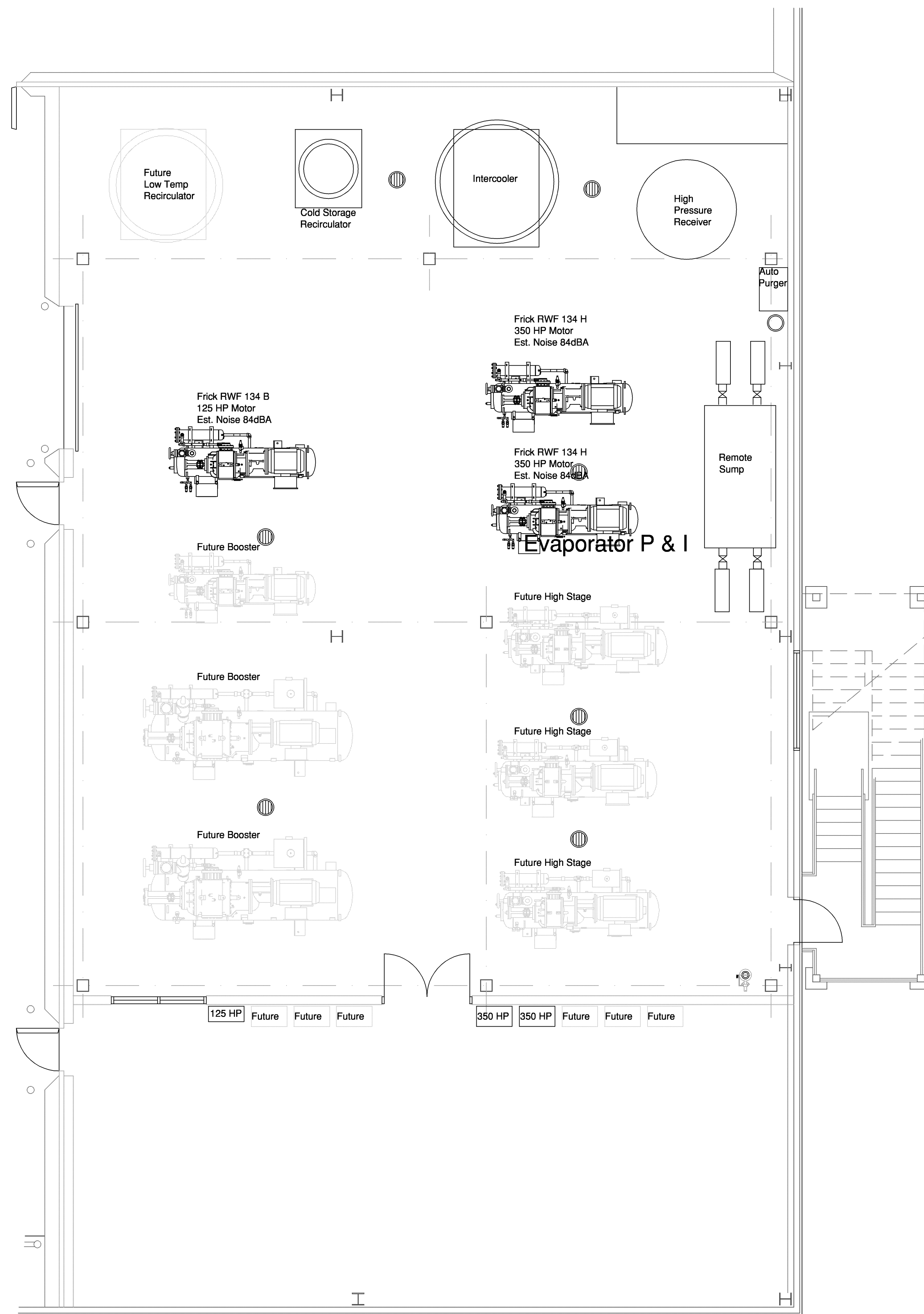
Plan View Equipment Room
