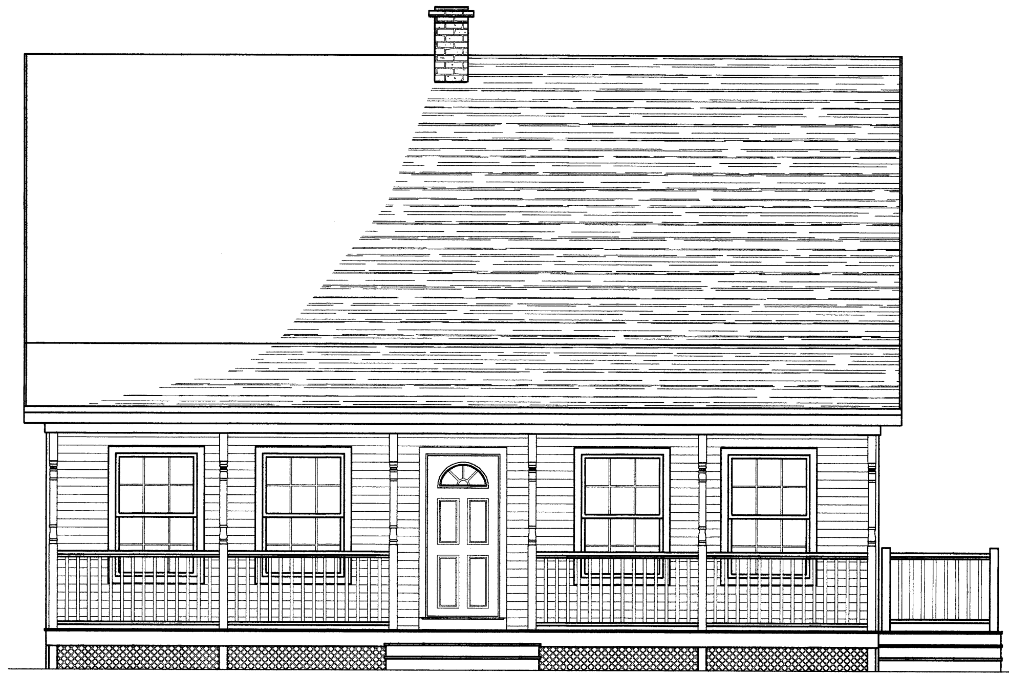
FRONT ELEVATION 1/4" = 1'-0"
