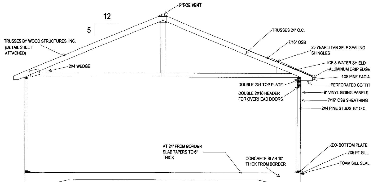
TYPICAL DETAIL
