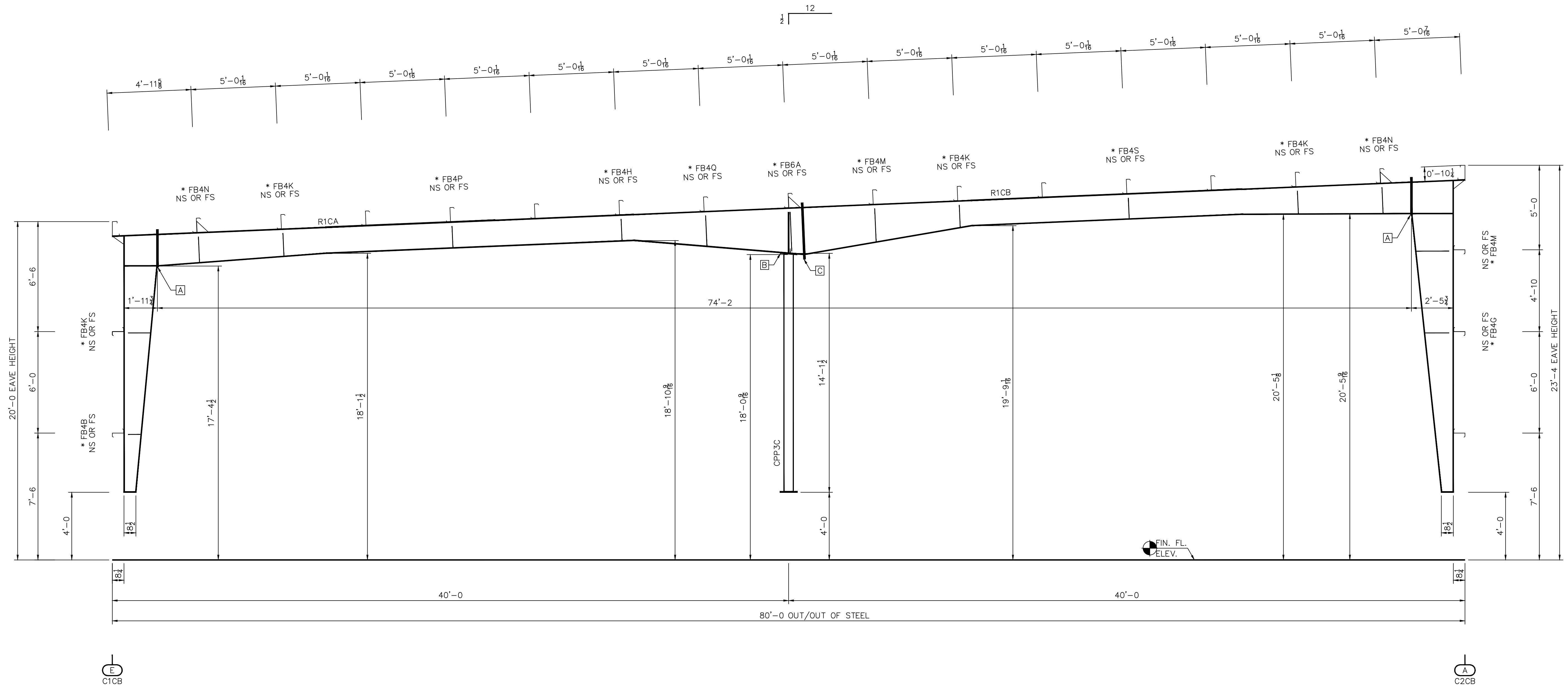
CROSS SECTION AT FRAME LINE "3"
