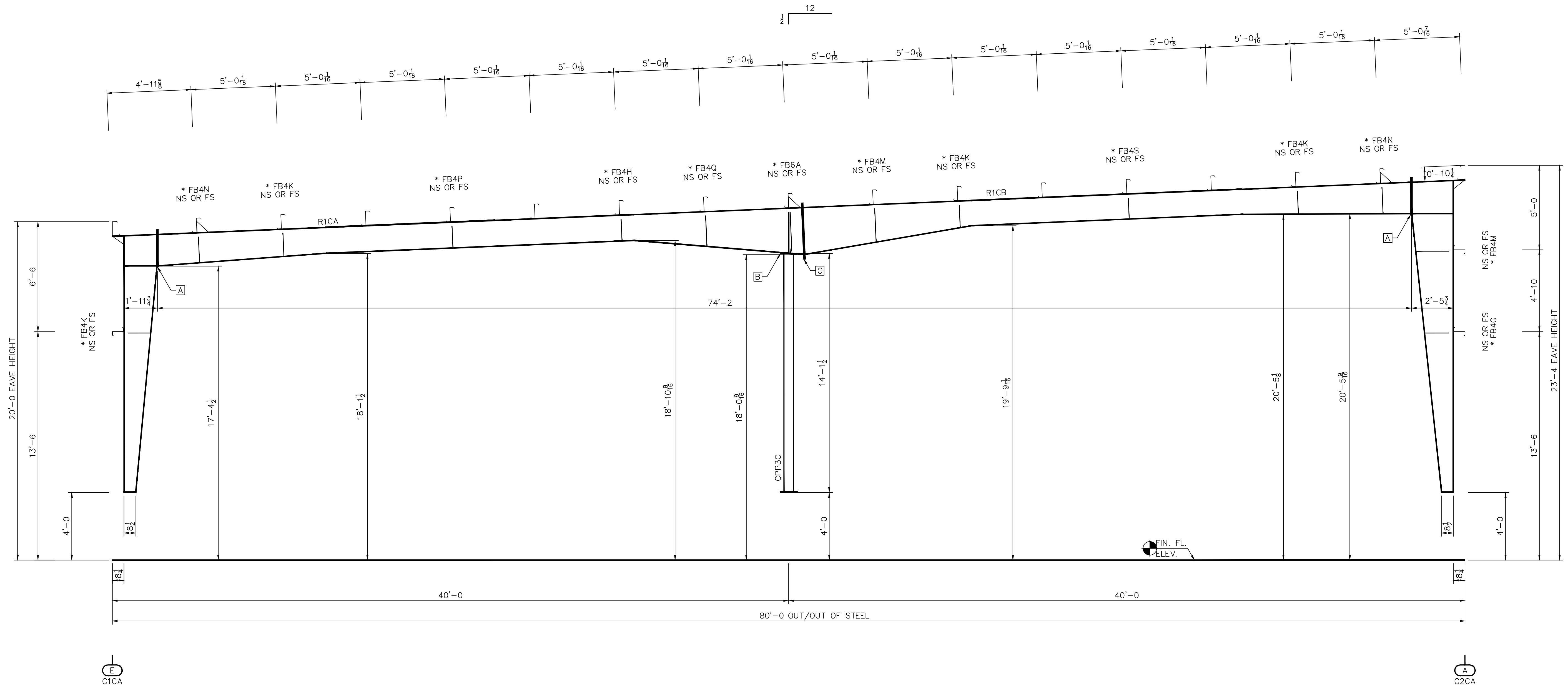
CROSS SECTION AT FRAME LINE "4"
