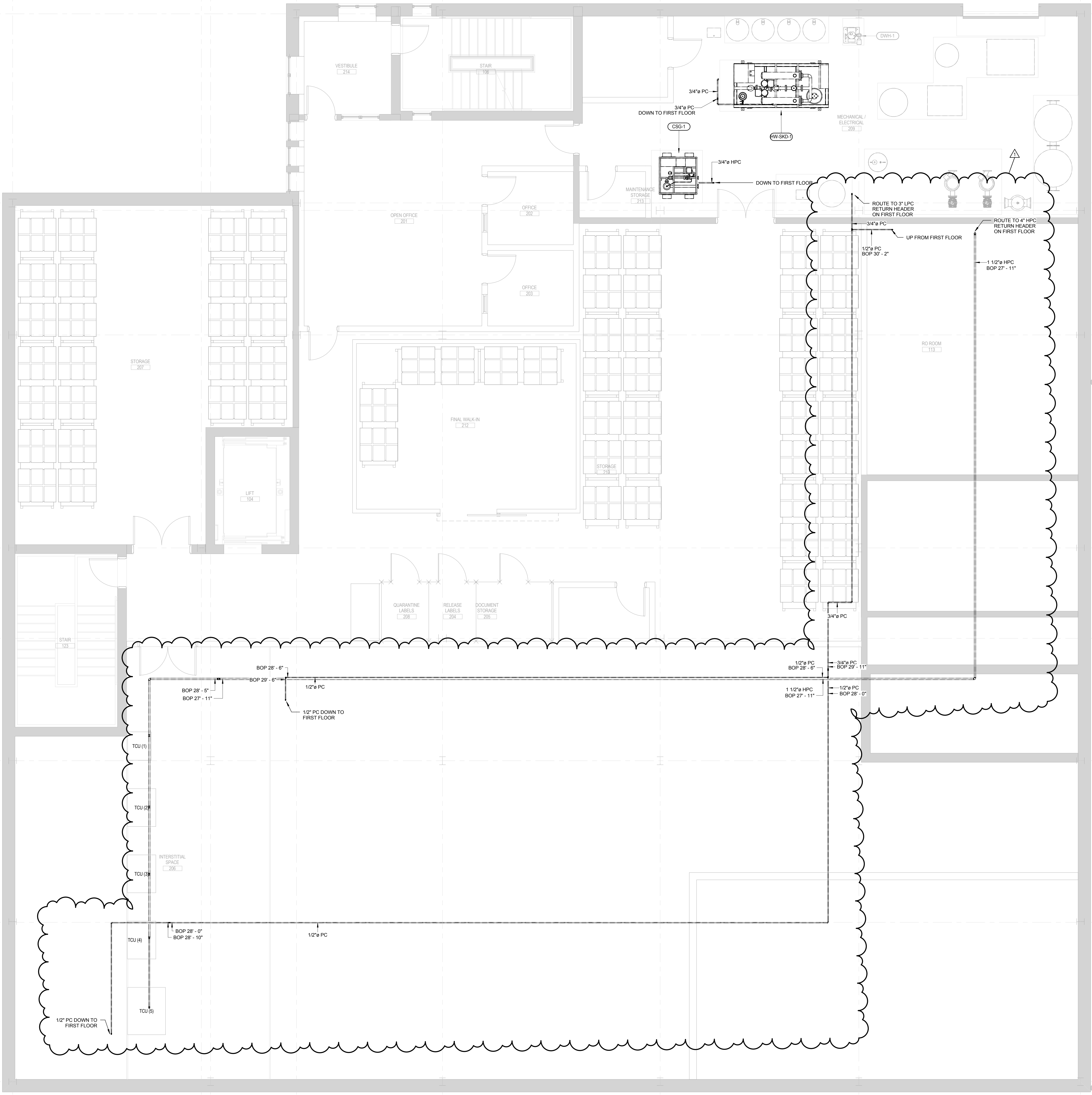
1 SECOND FLOOR - CONDENSATE PIPING PLAN MP-402-C 1/4" = 1'-0"
