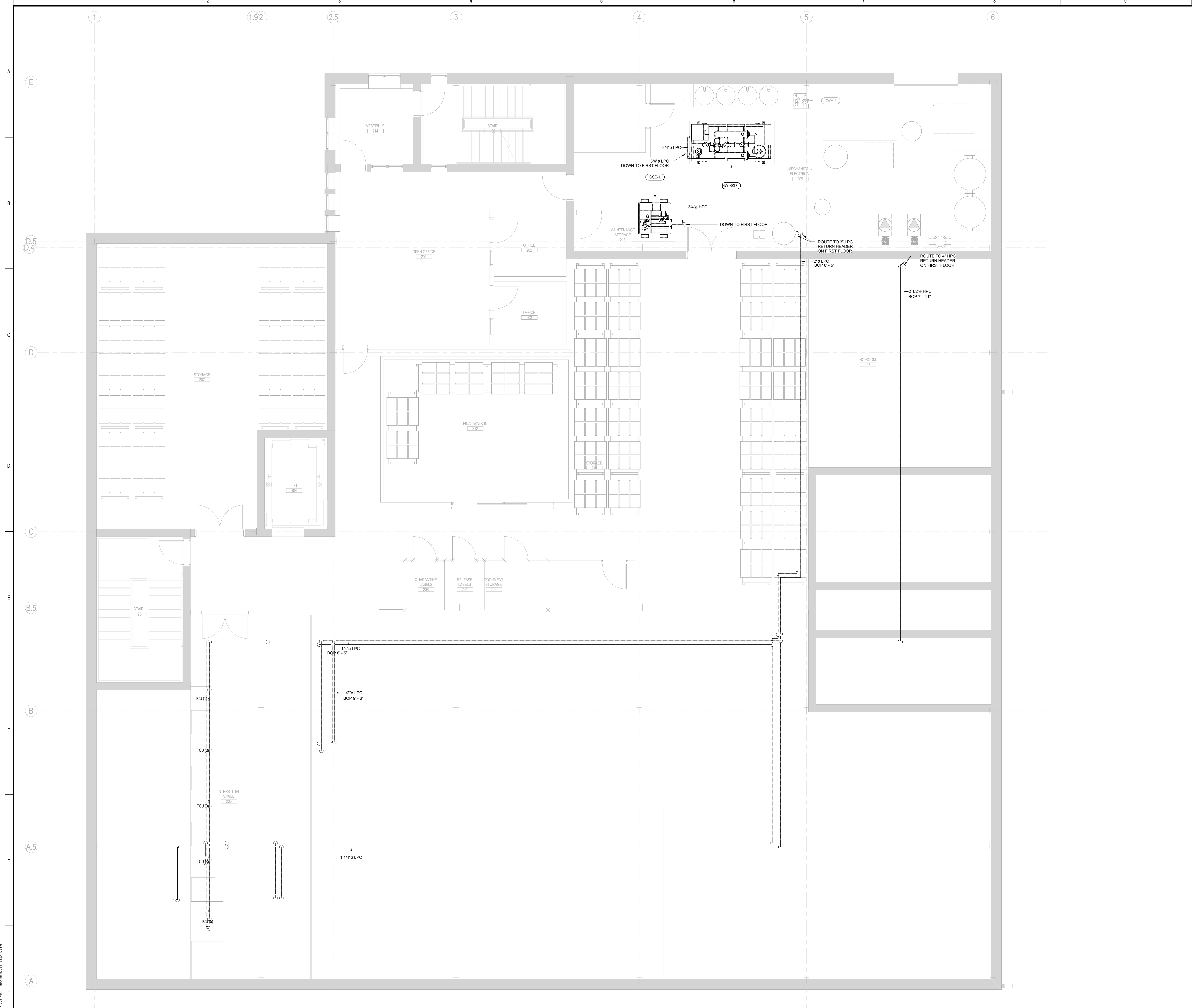
1 SECOND FLOOR - CONDENSATE PIPING PLAN 1/4" = 1'-0"
