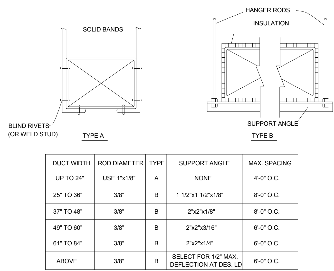
5 DUCTWORK HANGER DETAIL AND SCHEDULE MH-801-C N.T.S.
