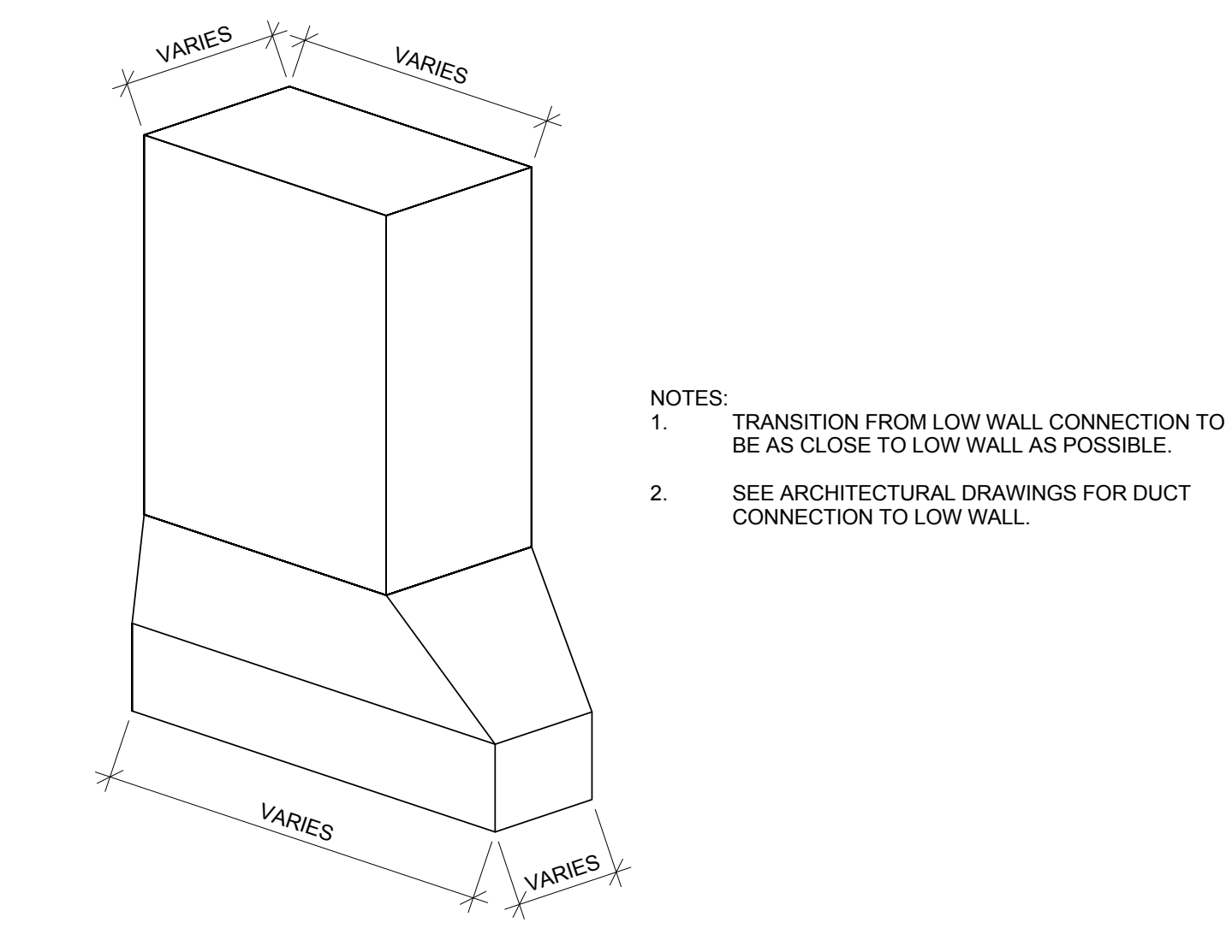
12 TYPICAL LOW WALL CONNECTION DETAIL MH-801-C N.T.S.
