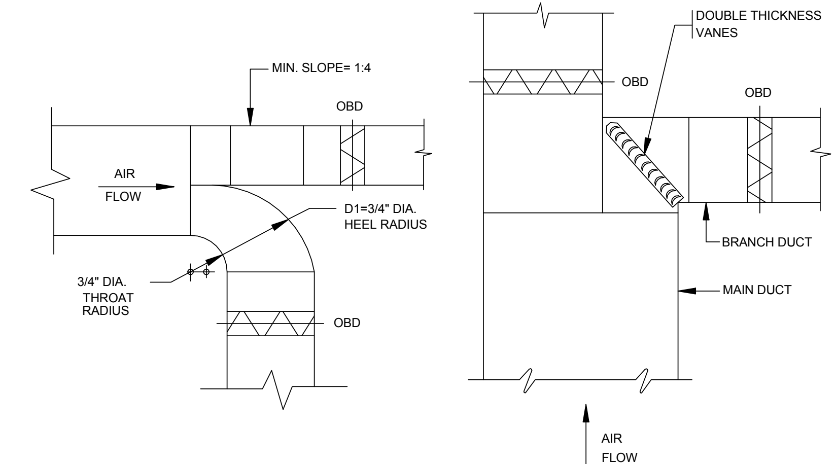
11 TYPICAL DUCT SPLITTER DETAIL MH-801-C N.T.S.
