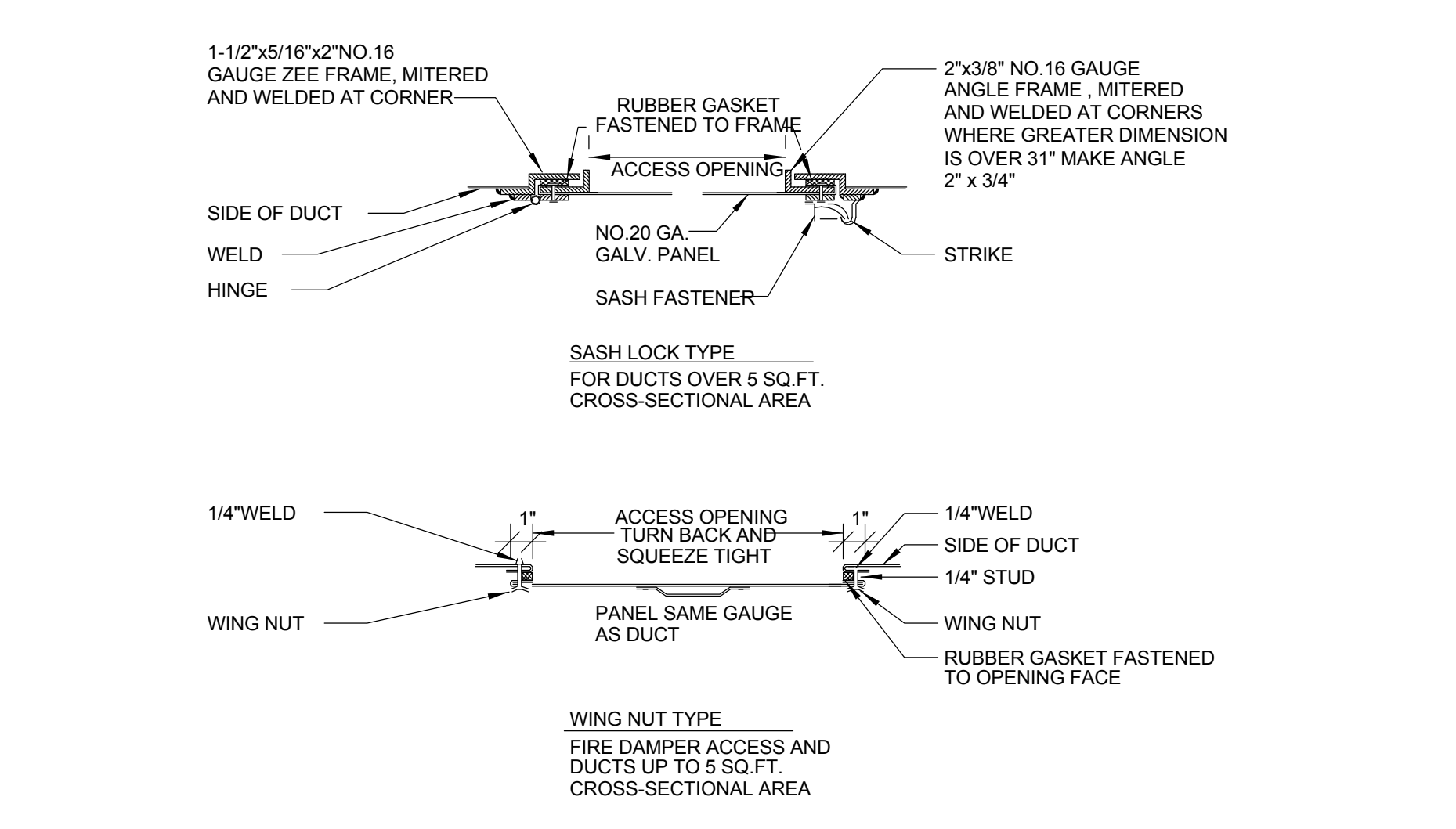
4 DUCTWORK ACCESS PANEL INSTALL DETAIL - UNINSULATED DUCT MH-801-C N.T.S.
