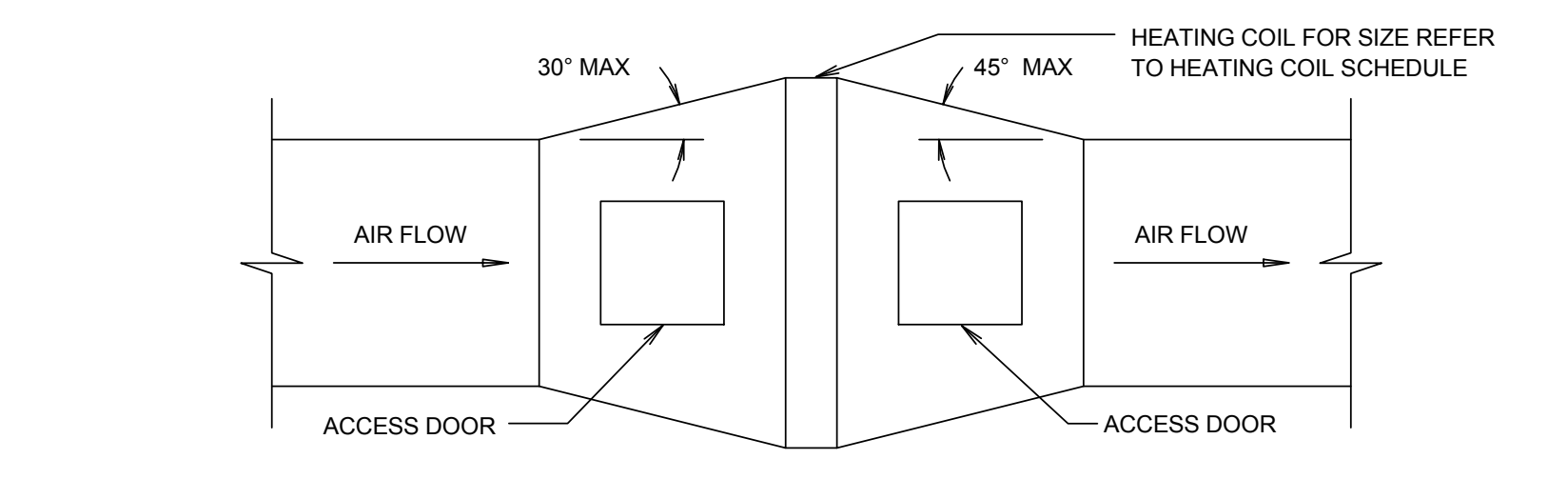
15 TYPICAL DUCT CONNECTION AT RE-HEATING COILS MH-801-C N.T.S.
