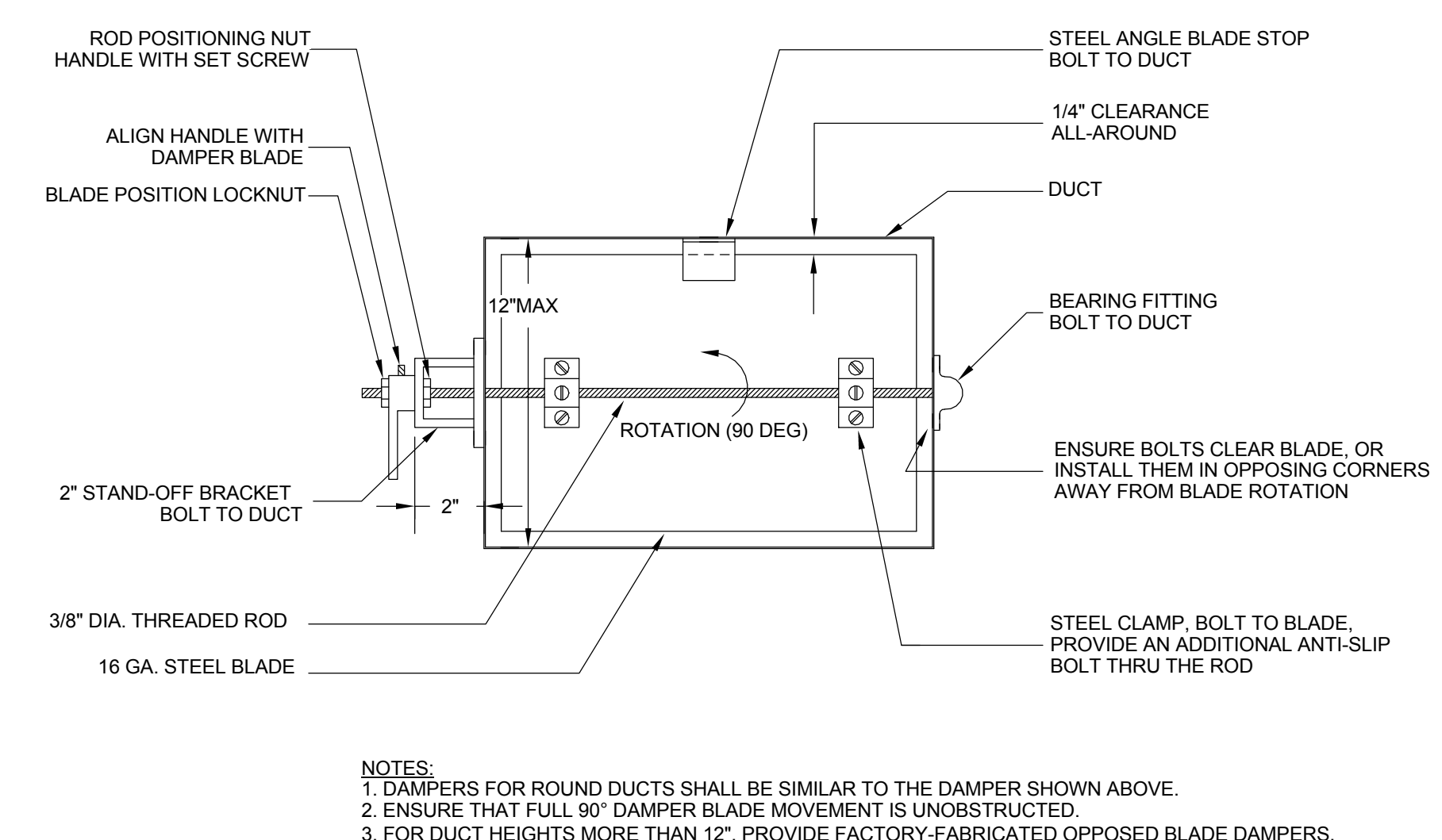
3 MANUAL DAMPER (ADJUSTABLE SINGLE-BLADE BALANCING TYPE) MH-801-C N.T.S.
