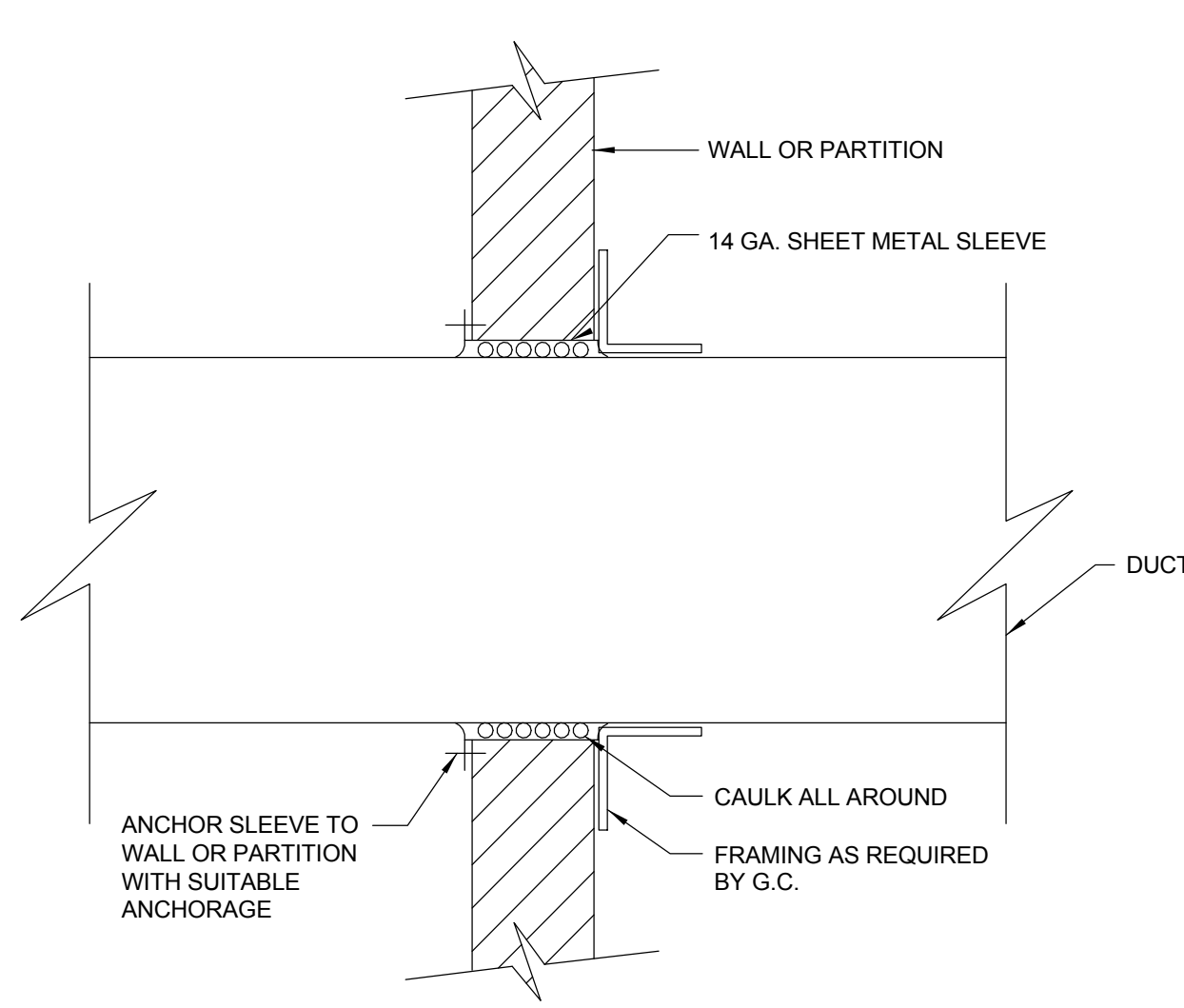
1 DUCT PENETRATION THRU WALL DETAIL MH-801-C N.T.S.
