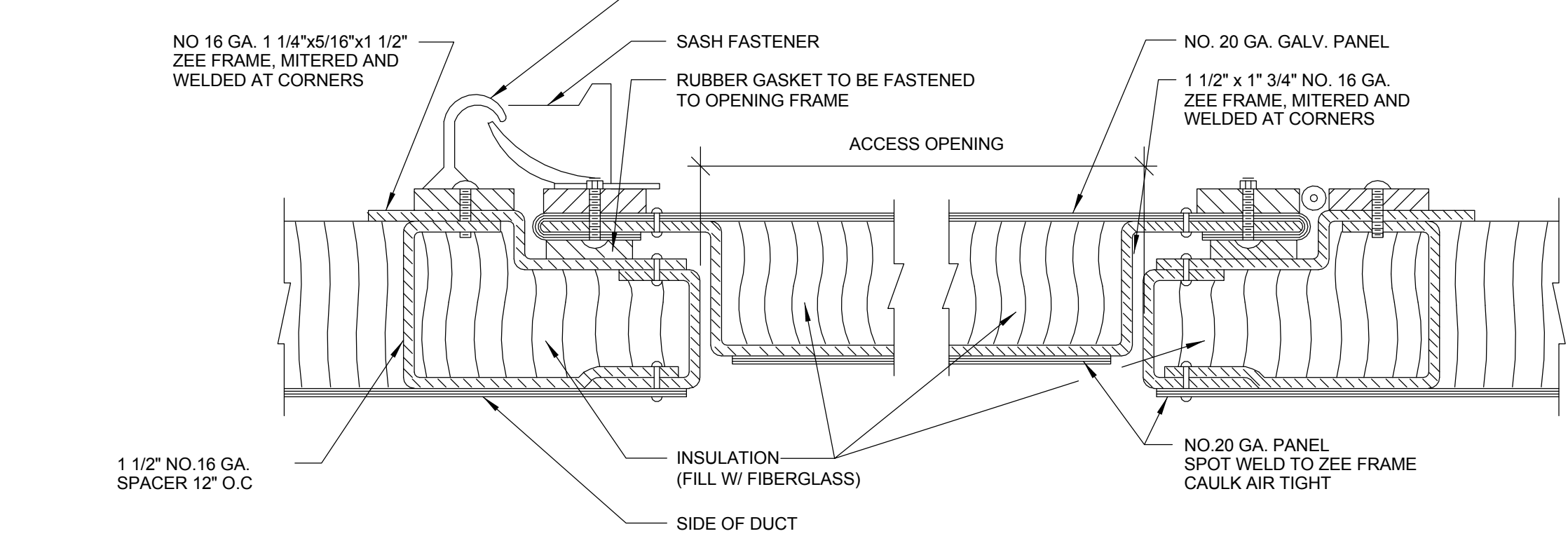
7 DUCTWORK ACCESS PANEL INSTALLATION DETAIL - INSULATED DUCT MH-801-C N.T.S.
