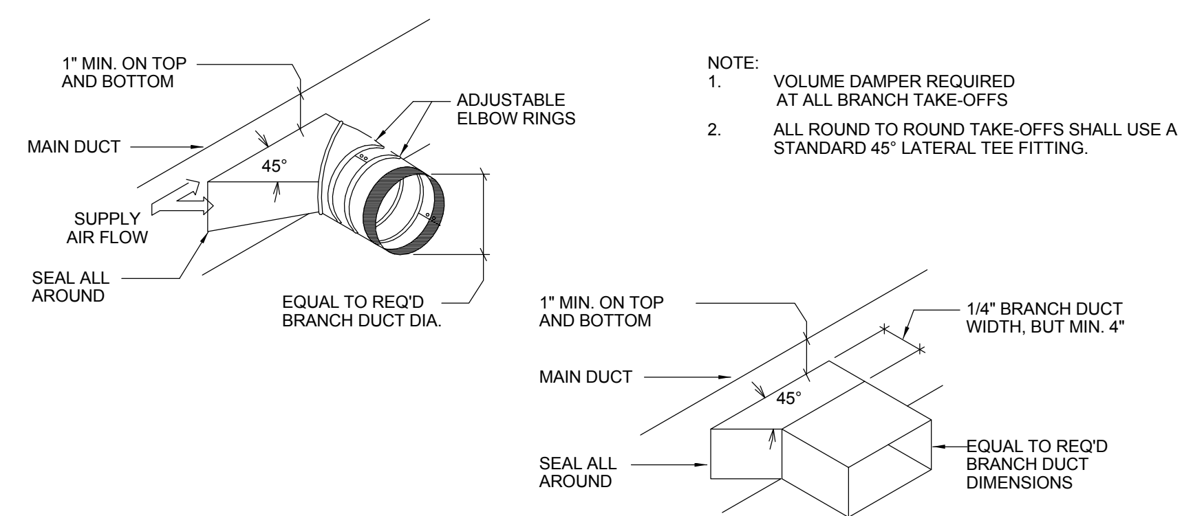
8 TYPICAL BRANCH TAKE-OFF FITTING DETAIL MH-801-C N.T.S.
