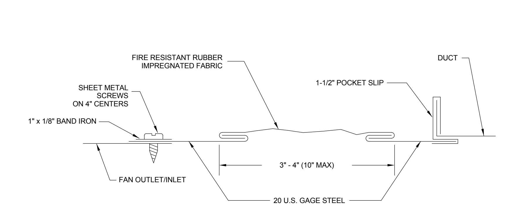
9 TYPICAL FLEXIBLE CONNECTION DETAIL MH-801-C N.T.S.
